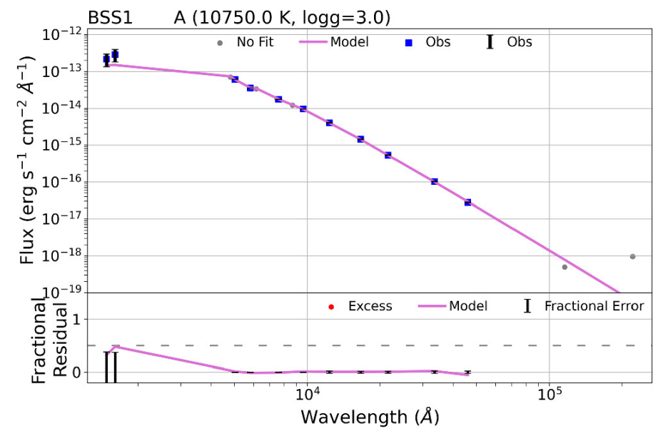
Figure 5. from Pinapati Saketh et al 2024 Astron. J. 168 doi:10.3847/1538-3881/ad5a96 https://dx.doi.org/10.3847/1538-3881/ad5a96 © 2024. The Author(s). Published by the American Astronomical Society.
