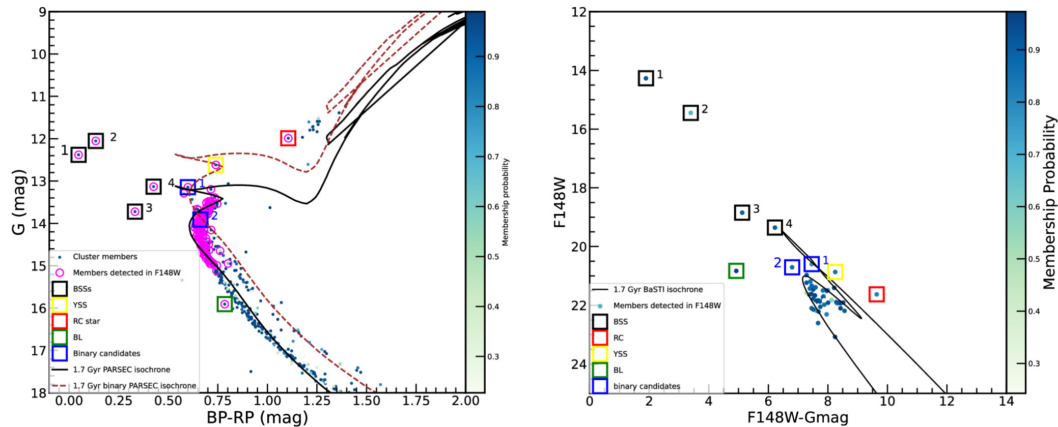
Figure 2. from Pinapati Saketh et al 2024 Astron. J. 168 doi:10.3847/1538-3881/ad5a96 https://dx.doi.org/10.3847/1538-3881/ad5a96 © 2024. The Author(s). Published by the American Astronomical Society.
