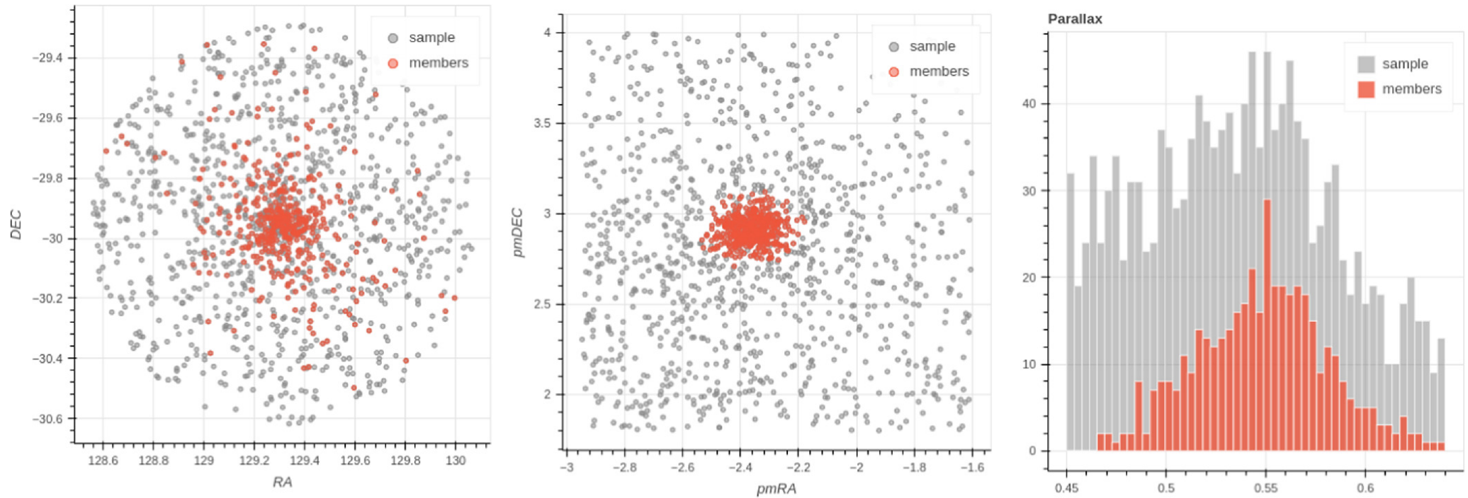
Figure 1. from Pinapati Saketh et al 2024 Astron. J. 168 doi:10.3847/1538-3881/ad5a96 https://dx.doi.org/10.3847/1538-3881/ad5a96 © 2024. The Author(s). Published by the American Astronomical Society.
