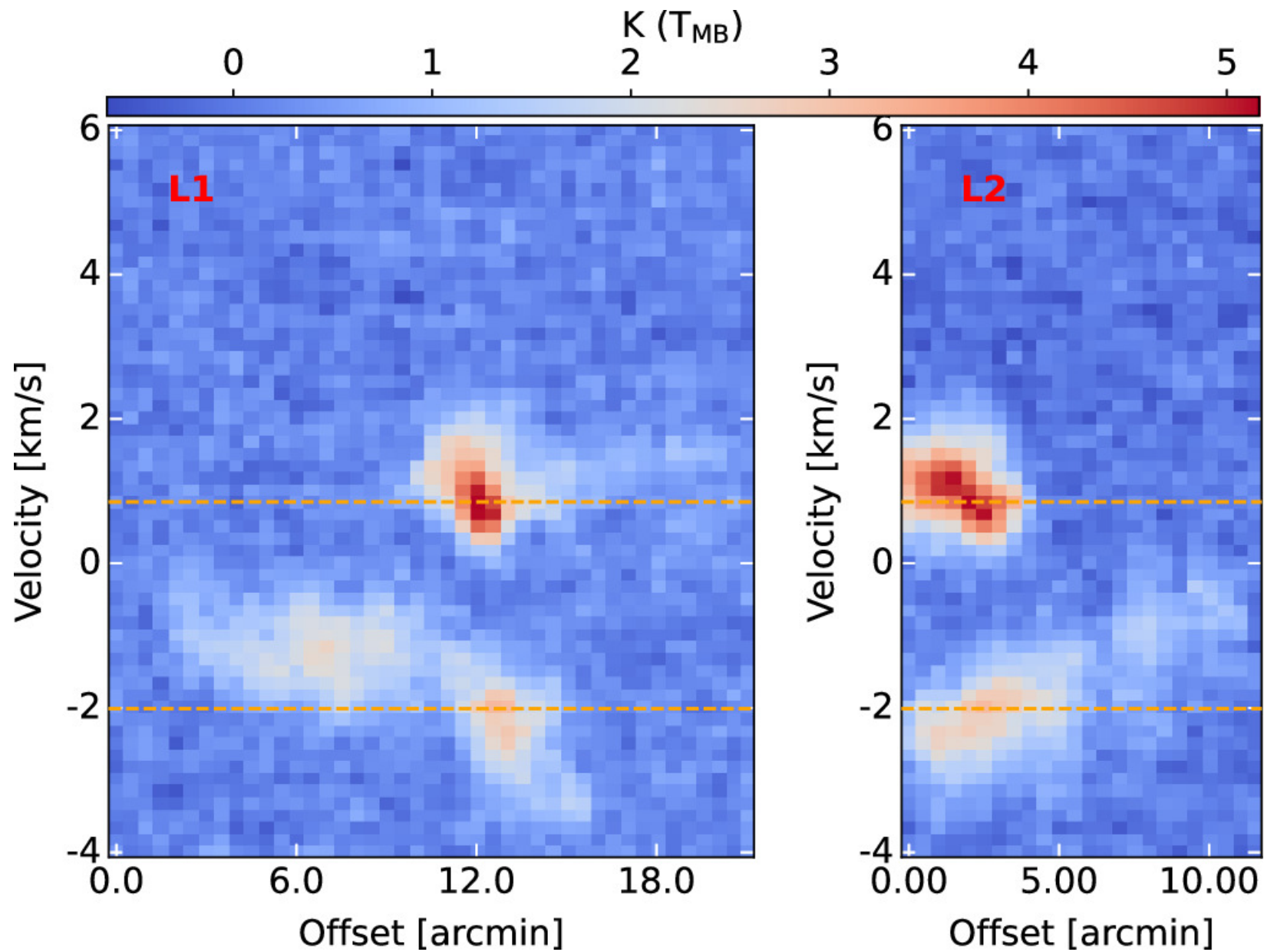
Figure 9. from Aayushi Verma et al 2024 Astron. J. 168 doi:10.3847/1538-3881/ad5a8b https://dx.doi.org/10.3847/1538-3881/ad5a8b © 2024. The Author(s). Published by the American Astronomical Society.
