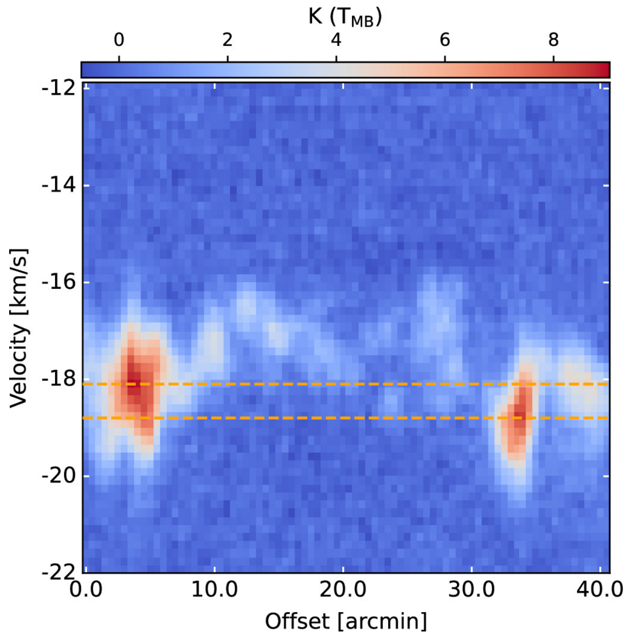
Figure 5. from Aayushi Verma et al 2024 Astron. J. 168 doi:10.3847/1538-3881/ad5a8b https://dx.doi.org/10.3847/1538-3881/ad5a8b © 2024. The Author(s). Published by the American Astronomical Society.
