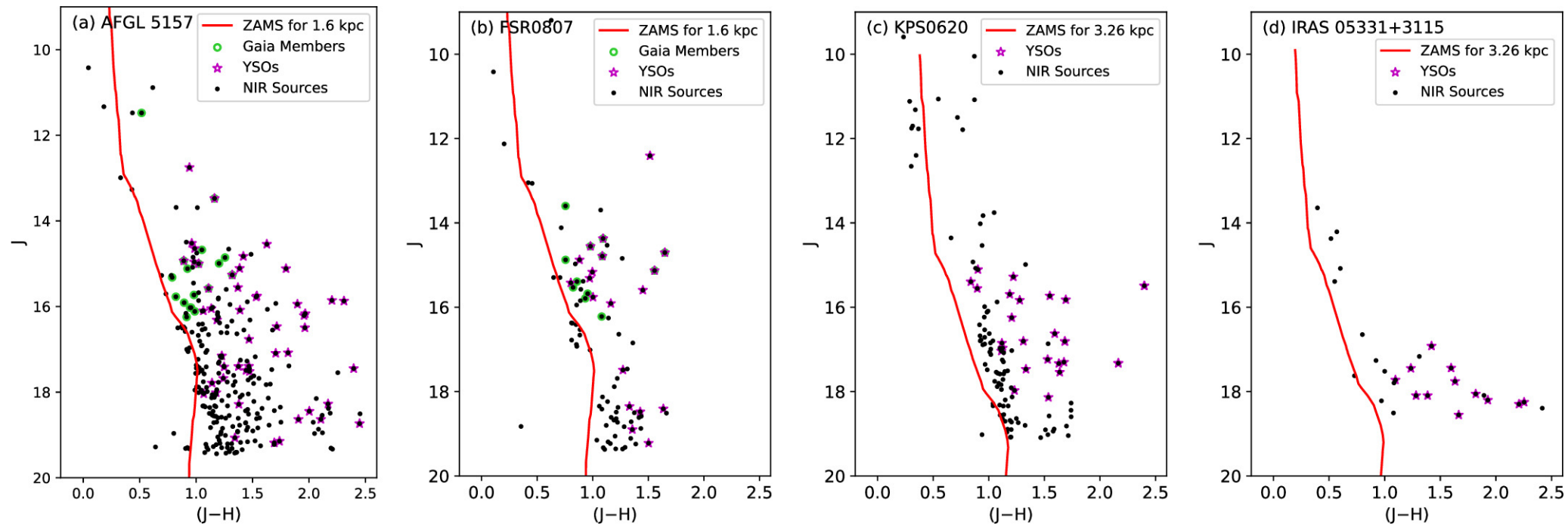
Figure 13. from Aayushi Verma et al 2024 Astron. J. 168 doi:10.3847/1538-3881/ad5a8b https://dx.doi.org/10.3847/1538-3881/ad5a8b © 2024. The Author(s). Published by the American Astronomical Society.
