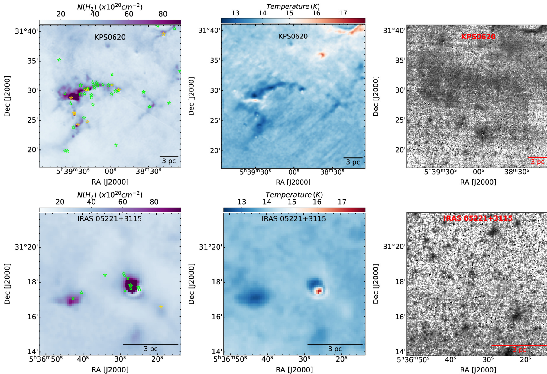
Figure 11. from Aayushi Verma et al 2024 Astron. J. 168 doi:10.3847/1538-3881/ad5a8b https://dx.doi.org/10.3847/1538-3881/ad5a8b © 2024. The Author(s). Published by the American Astronomical Society.
