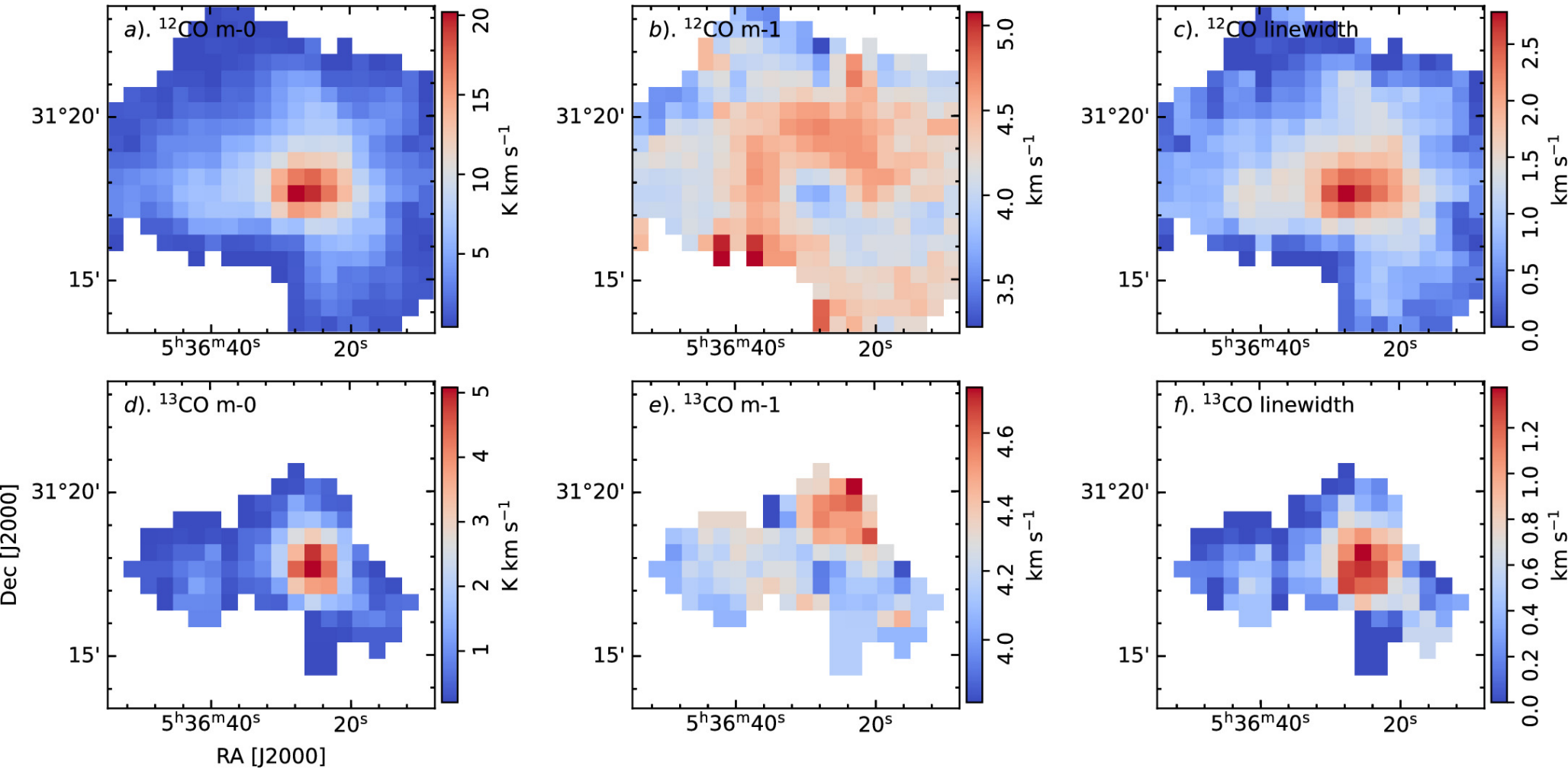
Figure 10. from Aayushi Verma et al 2024 Astron. J. 168 doi:10.3847/1538-3881/ad5a8b https://dx.doi.org/10.3847/1538-3881/ad5a8b © 2024. The Author(s). Published by the American Astronomical Society.
