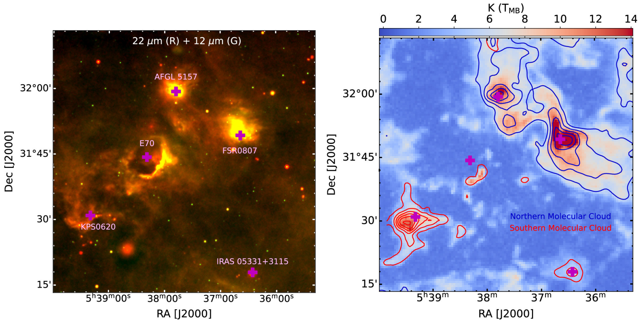
Figure 1. from Aayushi Verma et al 2024 Astron. J. 168 doi:10.3847/1538-3881/ad5a8b https://dx.doi.org/10.3847/1538-3881/ad5a8b © 2024. The Author(s). Published by the American Astronomical Society.
