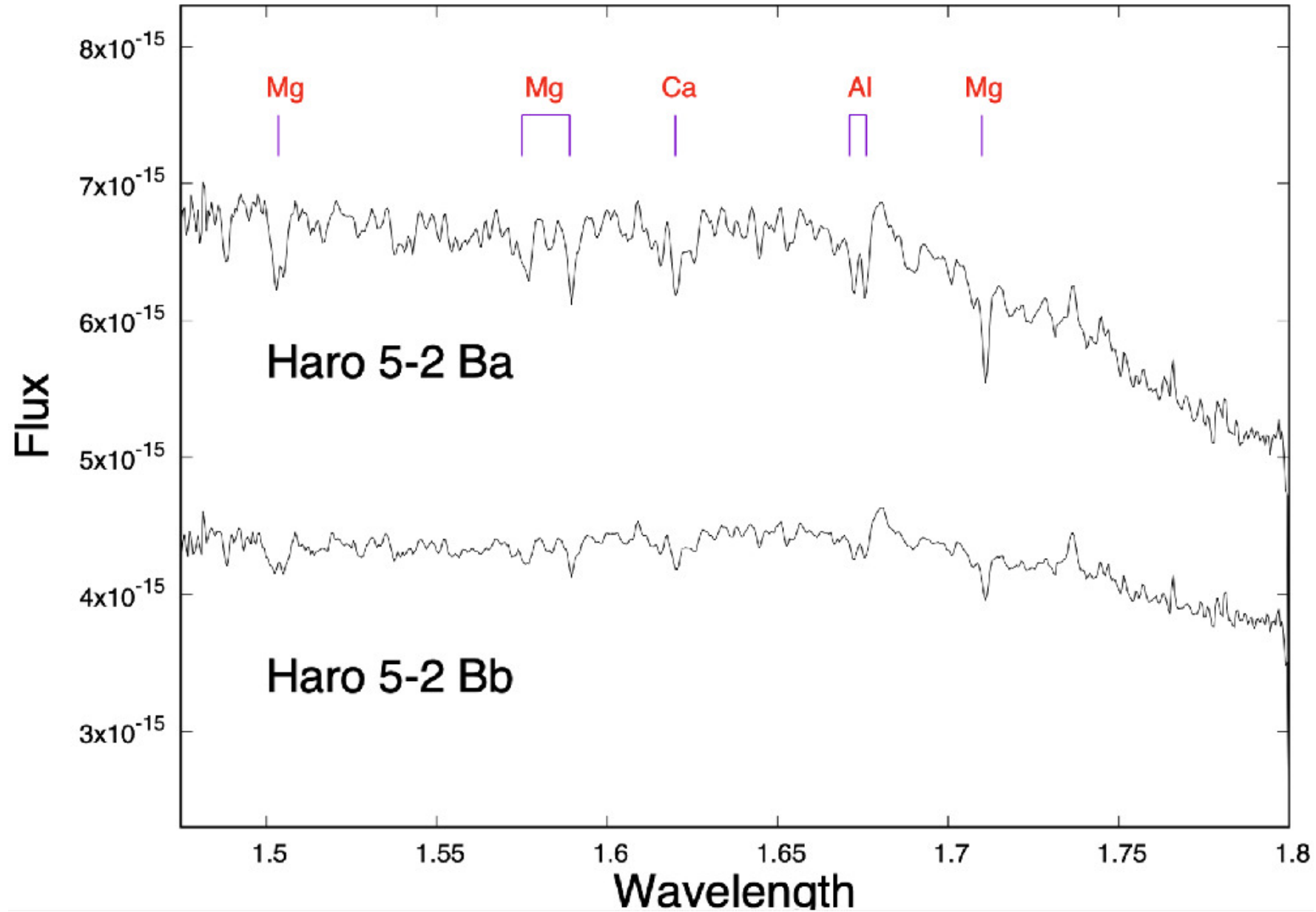
Figure 9. from Bo Reipurth et al 2024 Astron. J. 168 doi:10.3847/1538-3881/ad5956 https://dx.doi.org/10.3847/1538-3881/ad5956 © 2024. The Author(s). Published by the American Astronomical Society.
