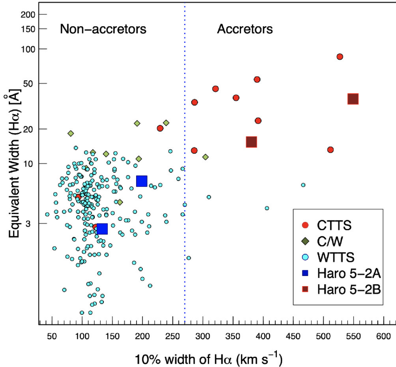
Figure 7. from Bo Reipurth et al 2024 Astron. J. 168 doi:10.3847/1538-3881/ad5956 https://dx.doi.org/10.3847/1538-3881/ad5956 © 2024. The Author(s). Published by the American Astronomical Society.
