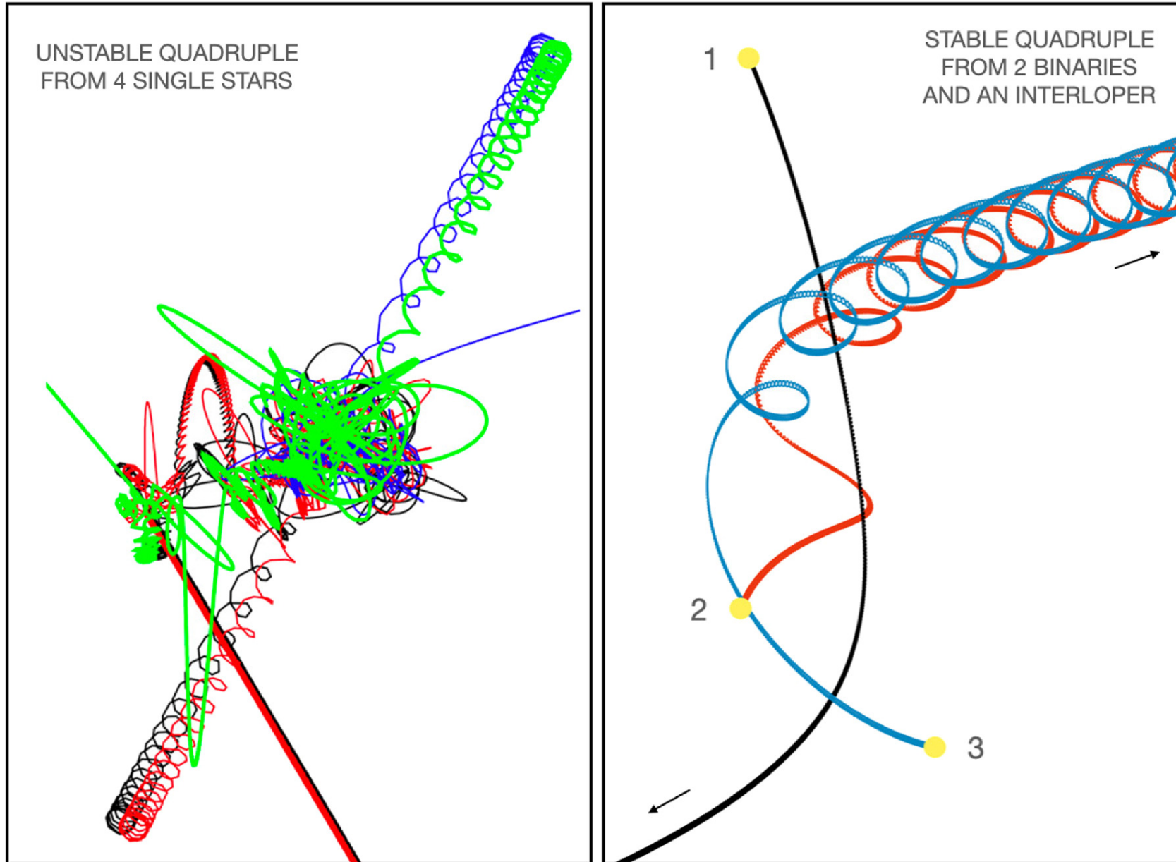
Figure 10. from Bo Reipurth et al 2024 Astron. J. 168 doi:10.3847/1538-3881/ad5956 https://dx.doi.org/10.3847/1538-3881/ad5956 © 2024. The Author(s). Published by the American Astronomical Society.
