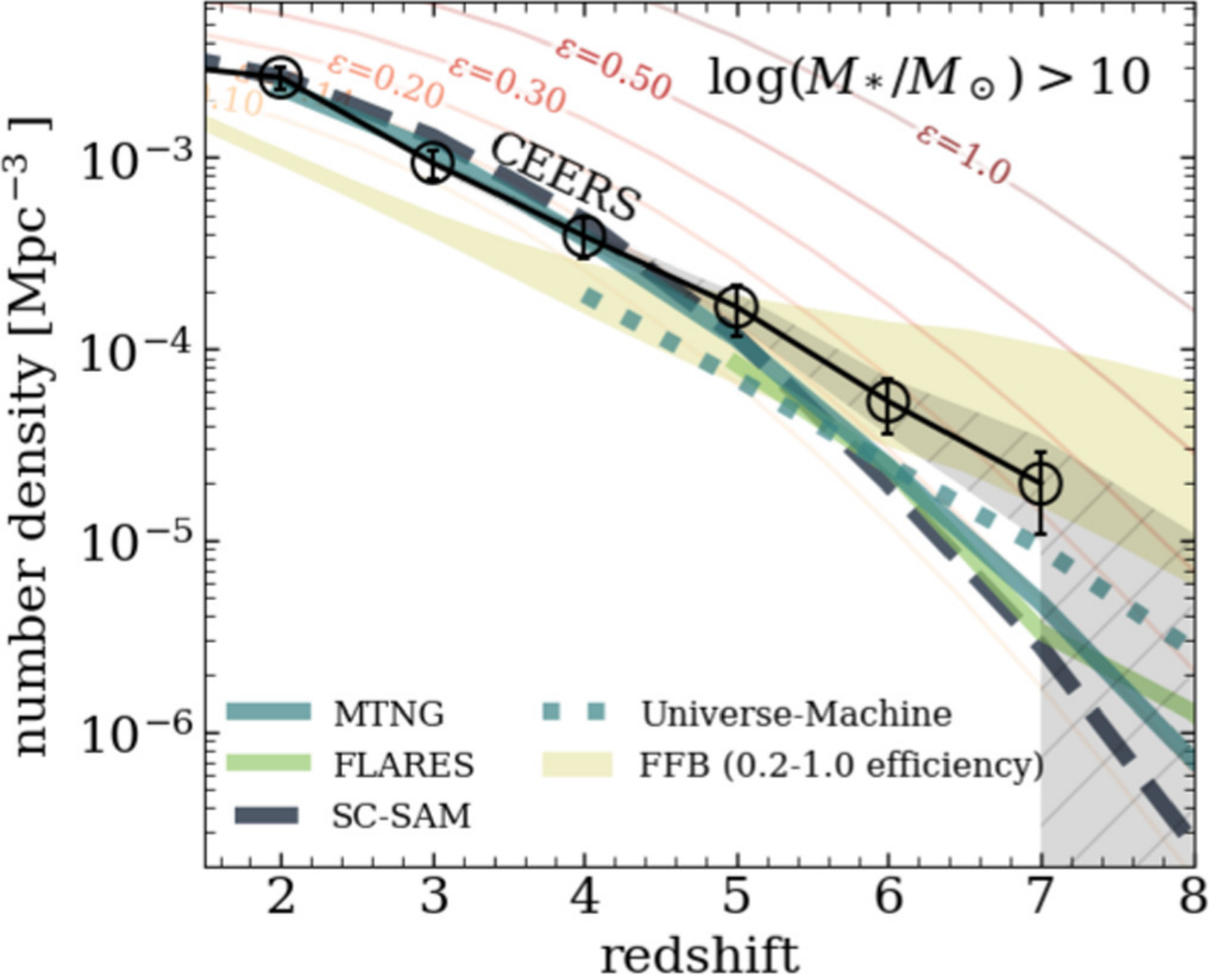
Figure 9. from Katherine Chworowsky et al 2024 Astron. J. 168 doi:10.3847/1538-3881/ad57c1 https://dx.doi.org/10.3847/1538-3881/ad57c1 © 2024. The Author(s). Published by the American Astronomical Society.
