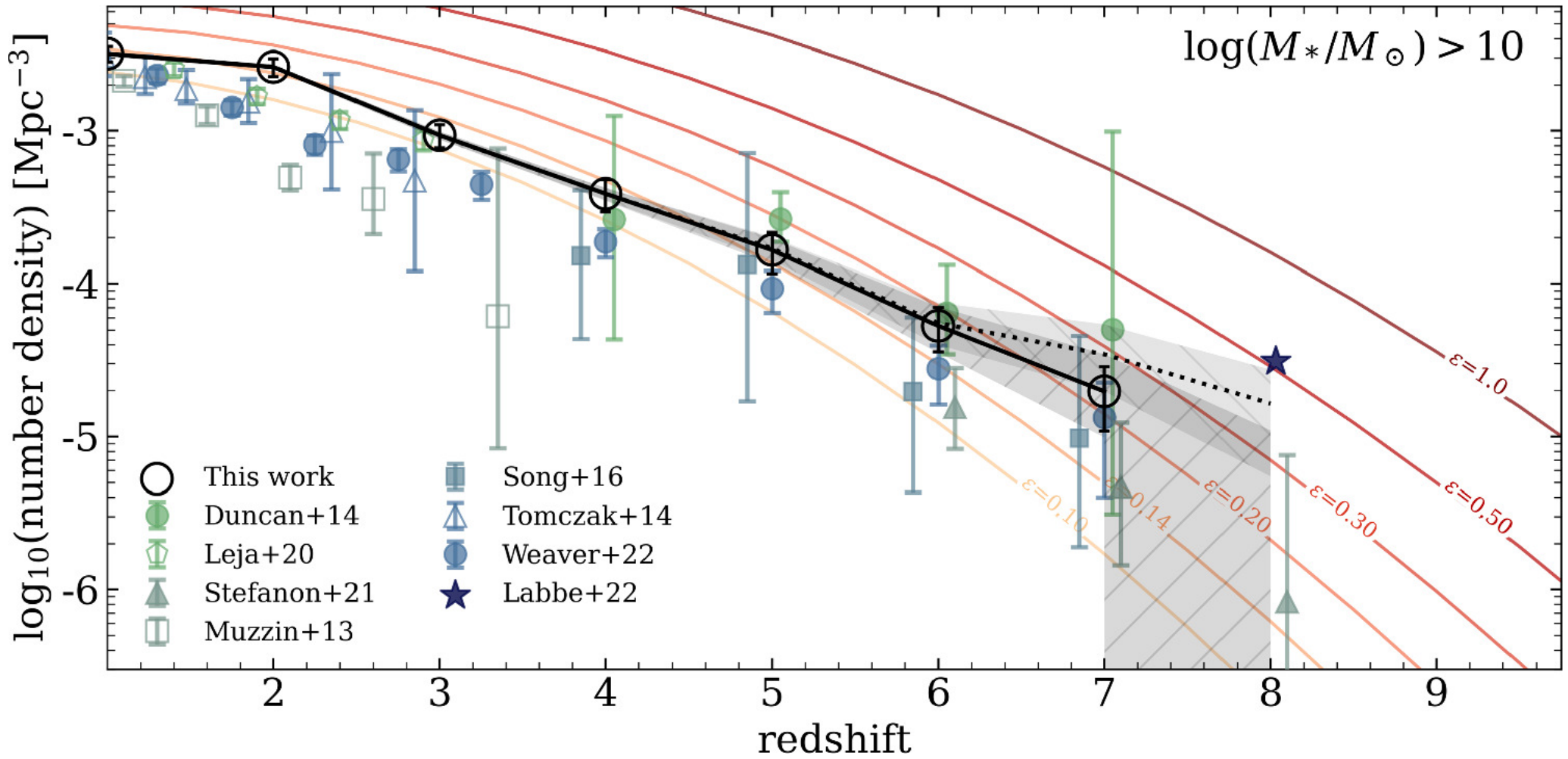
Figure 5. from Katherine Chworowsky et al 2024 Astron. J. 168 doi:10.3847/1538-3881/ad57c1 https://dx.doi.org/10.3847/1538-3881/ad57c1 © 2024. The Author(s). Published by the American Astronomical Society.
