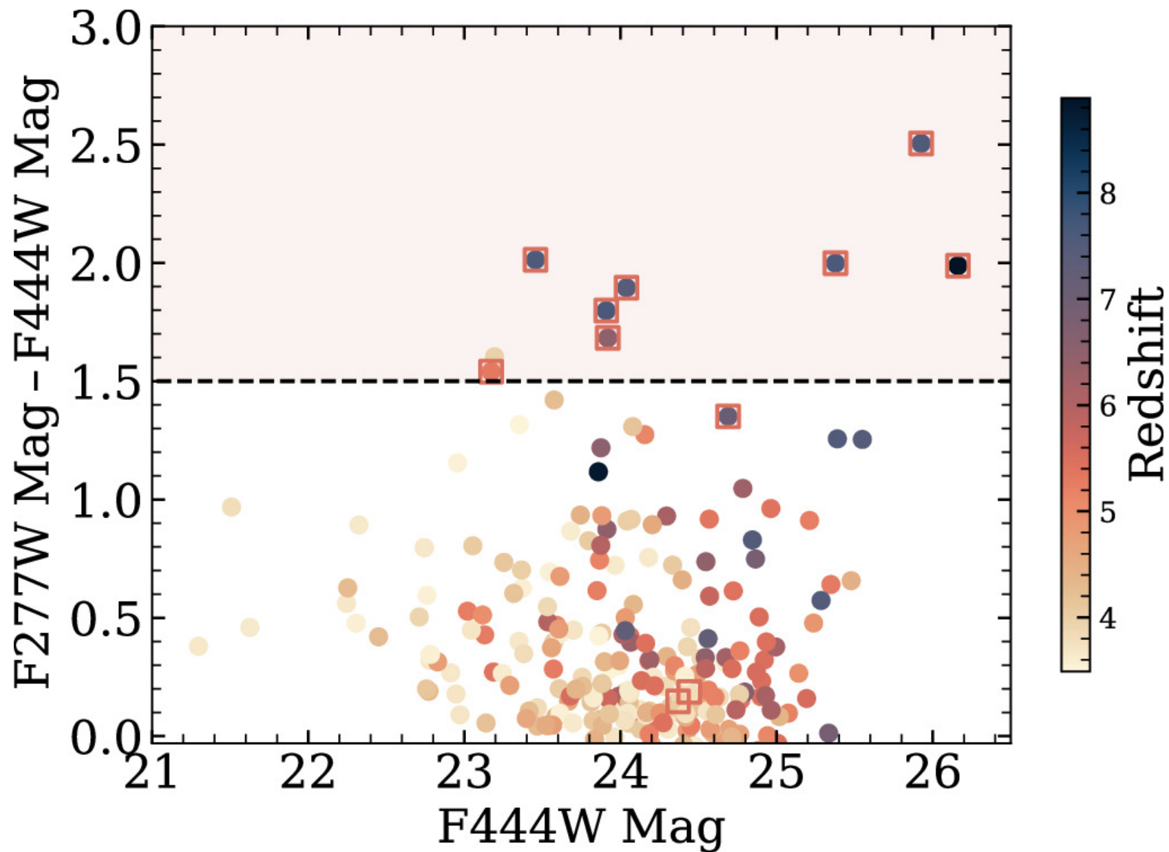
Figure 4. from Katherine Chworowsky et al 2024 Astron. J. 168 doi:10.3847/1538-3881/ad57c1 https://dx.doi.org/10.3847/1538-3881/ad57c1 © 2024. The Author(s). Published by the American Astronomical Society.
