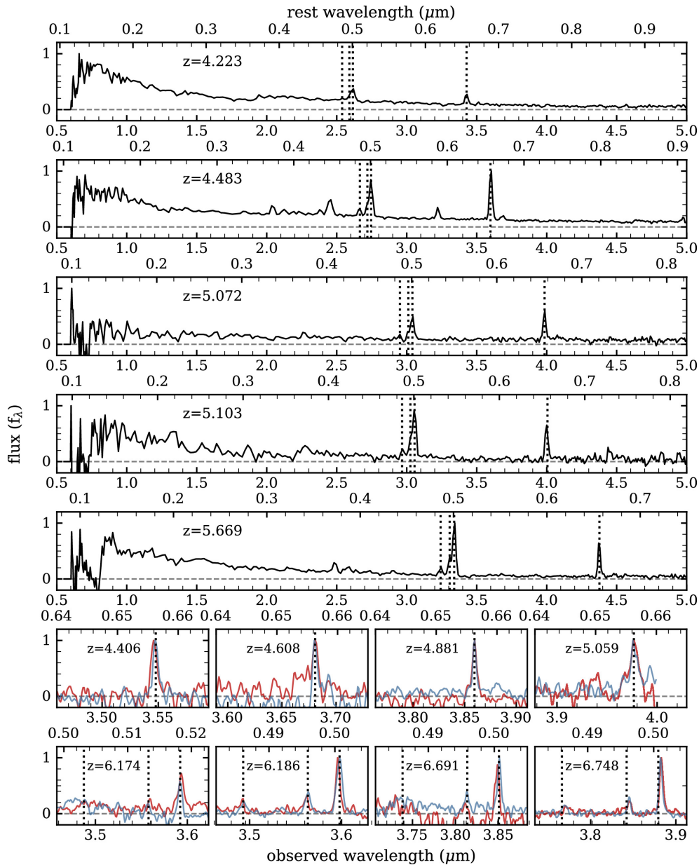
Figure 3. from Katherine Chworowsky et al 2024 Astron. J. 168 doi:10.3847/1538-3881/ad57c1 https://dx.doi.org/10.3847/1538-3881/ad57c1 © 2024. The Author(s). Published by the American Astronomical Society.
