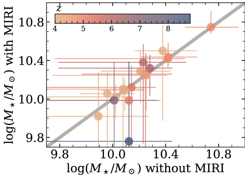
Figure 2. from Katherine Chworowsky et al 2024 Astron. J. 168 doi:10.3847/1538-3881/ad57c1 https://dx.doi.org/10.3847/1538-3881/ad57c1 © 2024. The Author(s). Published by the American Astronomical Society.
