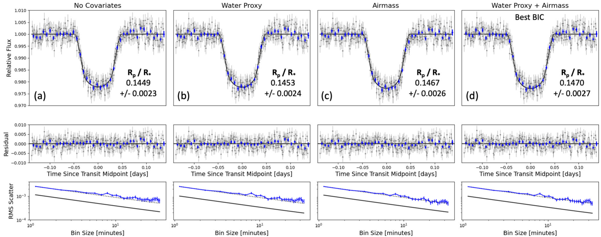
Figure 9. from W. Garrett Levine et al 2024 Astron. J. 168 doi:10.3847/1538-3881/ad5354 https://dx.doi.org/10.3847/1538-3881/ad5354 © 2024. The Author(s). Published by the American Astronomical Society.
