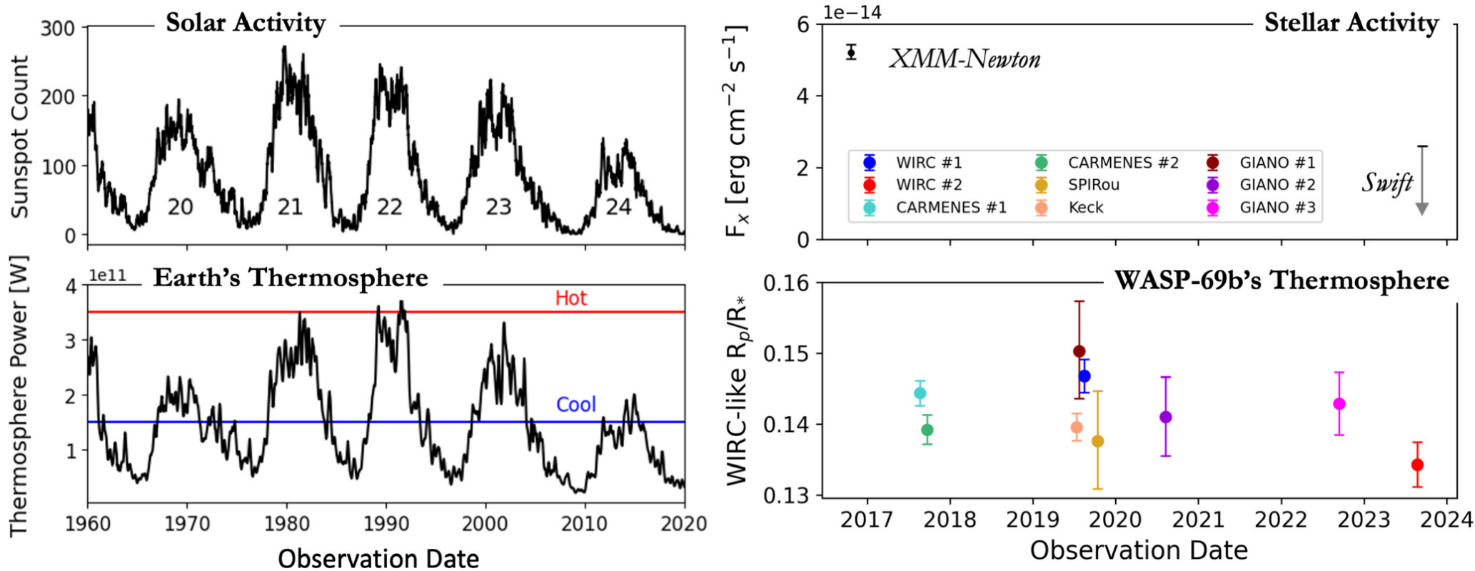
Figure 6. from W. Garrett Levine et al 2024 Astron. J. 168 doi:10.3847/1538-3881/ad5354 https://dx.doi.org/10.3847/1538-3881/ad5354 © 2024. The Author(s). Published by the American Astronomical Society.
