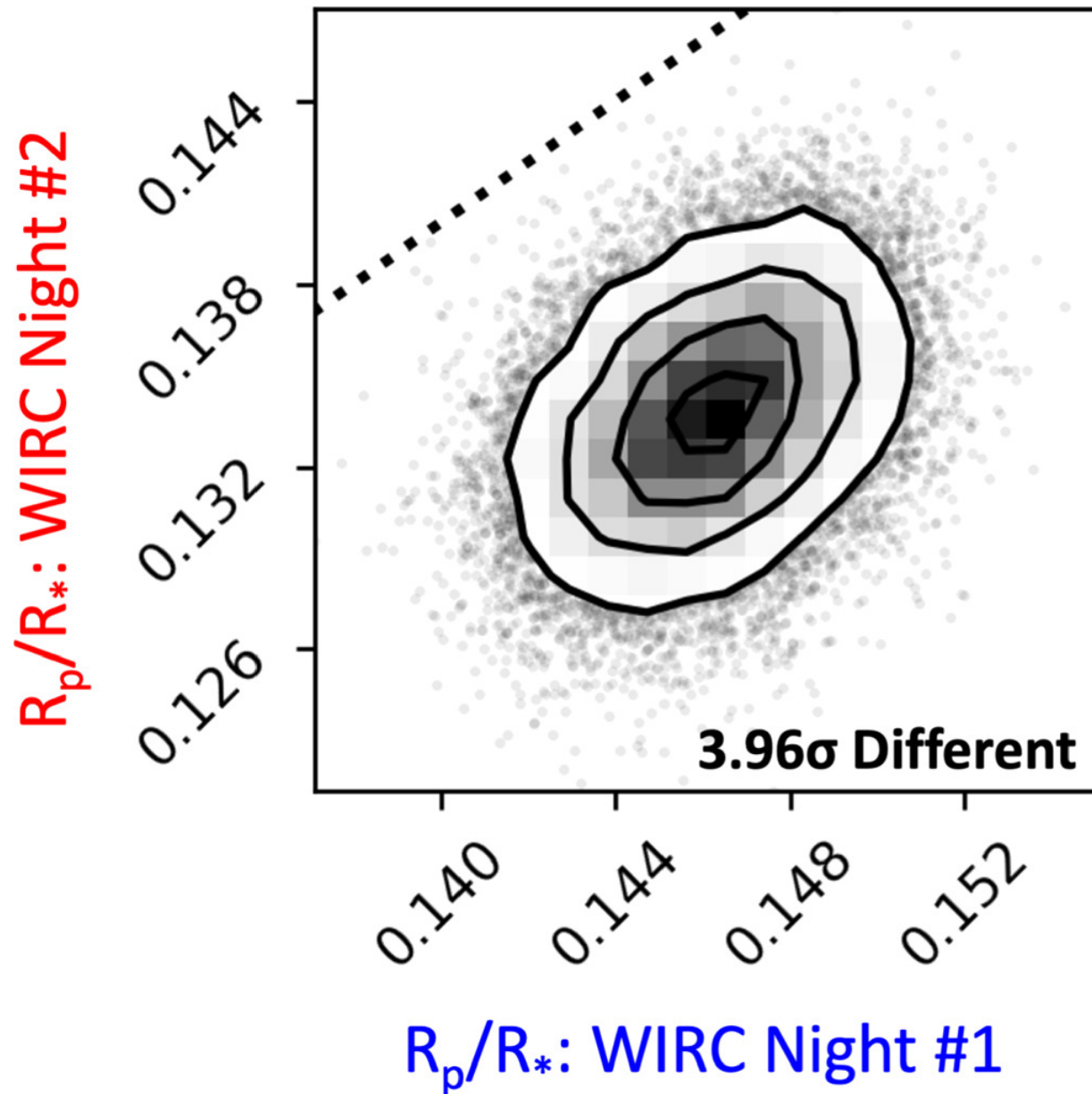
Figure 5. from W. Garrett Levine et al 2024 Astron. J. 168 doi:10.3847/1538-3881/ad5354 https://dx.doi.org/10.3847/1538-3881/ad5354 © 2024. The Author(s). Published by the American Astronomical Society.
