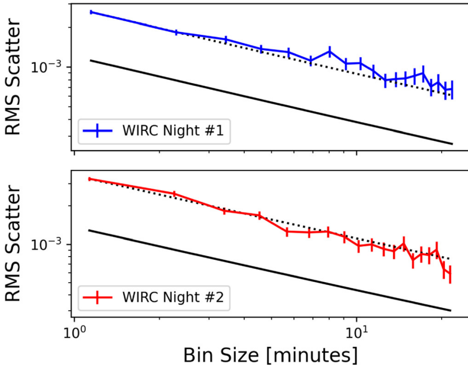
Figure 4. from W. Garrett Levine et al 2024 Astron. J. 168 doi:10.3847/1538-3881/ad5354 https://dx.doi.org/10.3847/1538-3881/ad5354 © 2024. The Author(s). Published by the American Astronomical Society.
