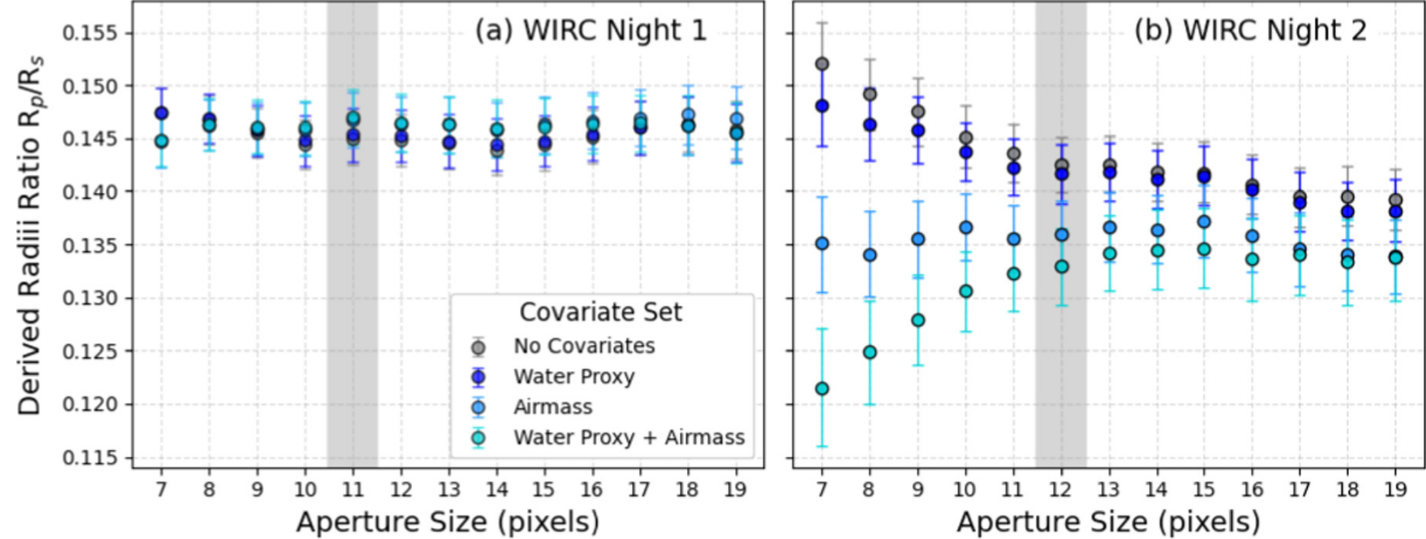
Figure 11. from W. Garrett Levine et al 2024 Astron. J. 168 doi:10.3847/1538-3881/ad5354 https://dx.doi.org/10.3847/1538-3881/ad5354 © 2024. The Author(s). Published by the American Astronomical Society.
