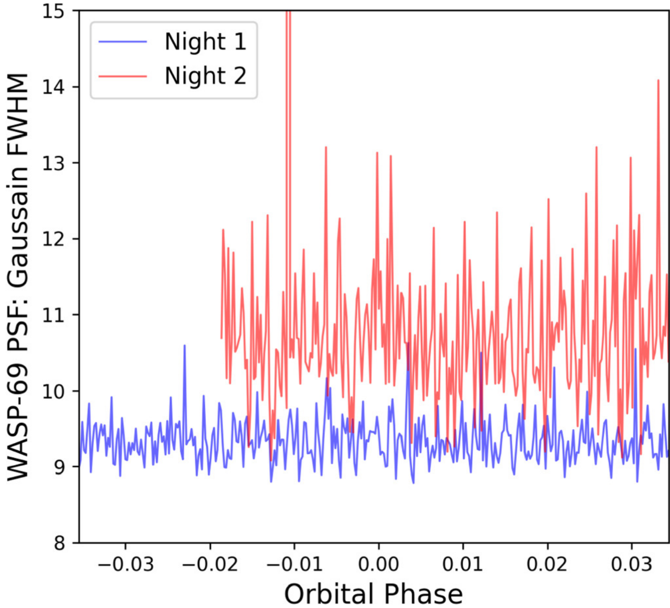
Figure 1. from W. Garrett Levine et al 2024 Astron. J. 168 doi:10.3847/1538-3881/ad5354 https://dx.doi.org/10.3847/1538-3881/ad5354 © 2024. The Author(s). Published by the American Astronomical Society.
