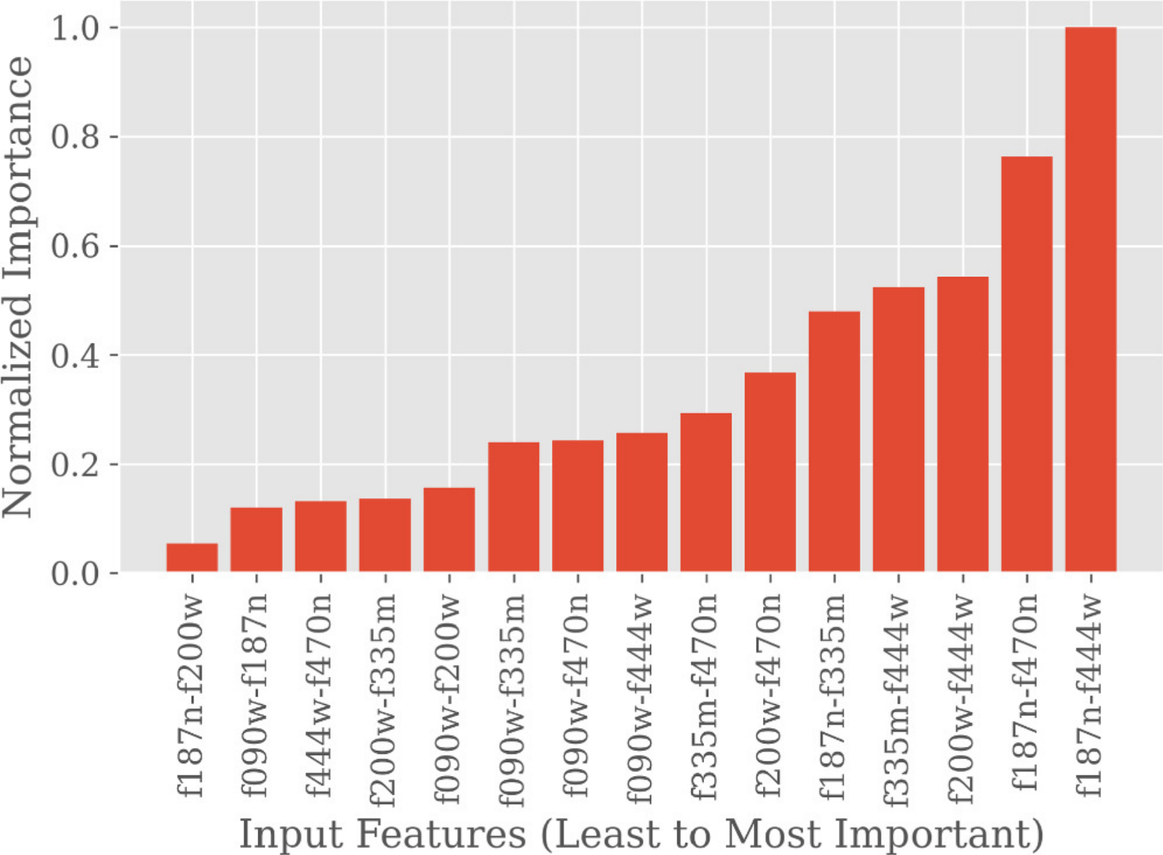
Figure 9. from B. L. Crompvoets et al 2024 Astron. J. 168 doi:10.3847/1538-3881/ad51fc https://dx.doi.org/10.3847/1538-3881/ad51fc © 2024. The Author(s). Published by the American Astronomical Society.
