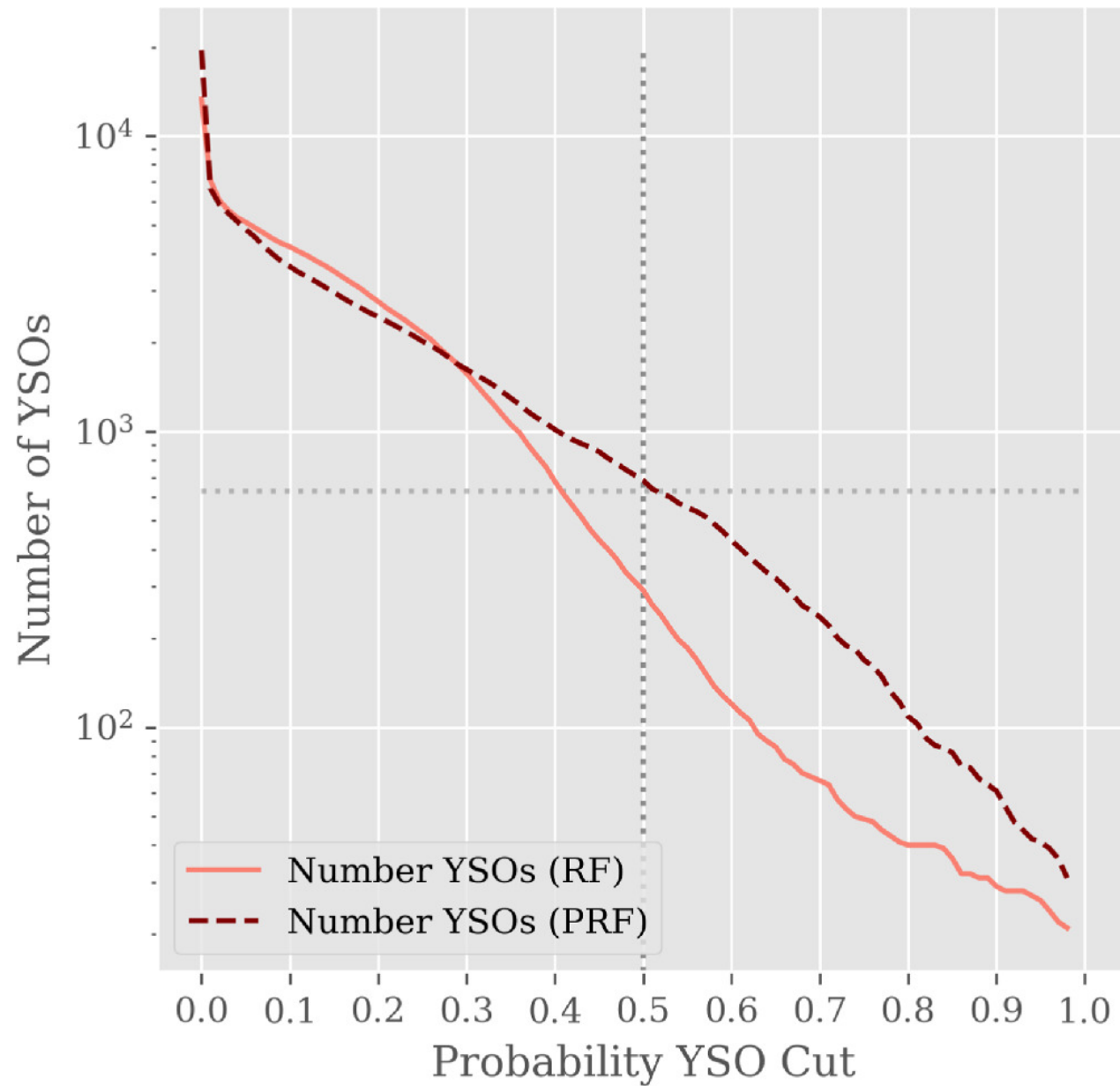
Figure 5. from B. L. Crompvoets et al 2024 Astron. J. 168 doi:10.3847/1538-3881/ad51fc https://dx.doi.org/10.3847/1538-3881/ad51fc © 2024. The Author(s). Published by the American Astronomical Society.
