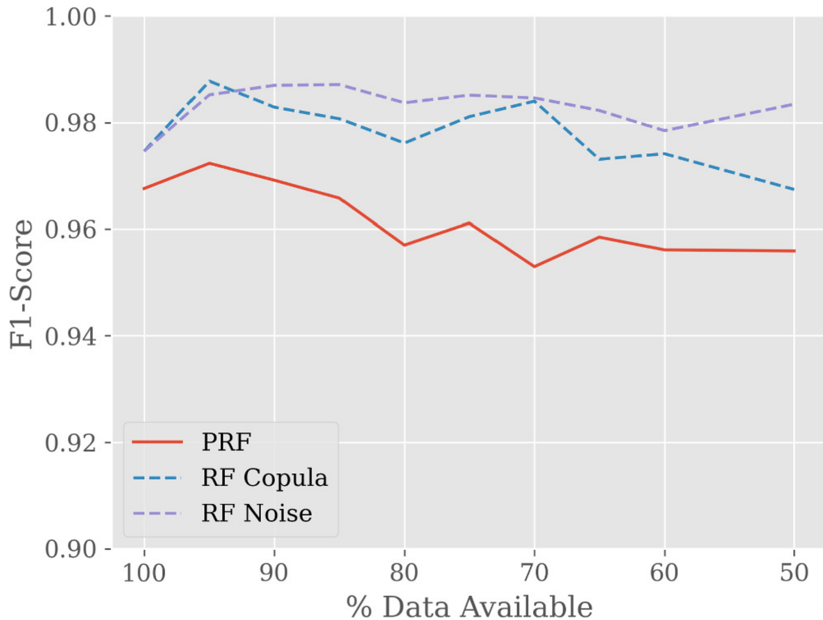
Figure 2. from B. L. Crompvoets et al 2024 Astron. J. 168 doi:10.3847/1538-3881/ad51fc https://dx.doi.org/10.3847/1538-3881/ad51fc © 2024. The Author(s). Published by the American Astronomical Society.
