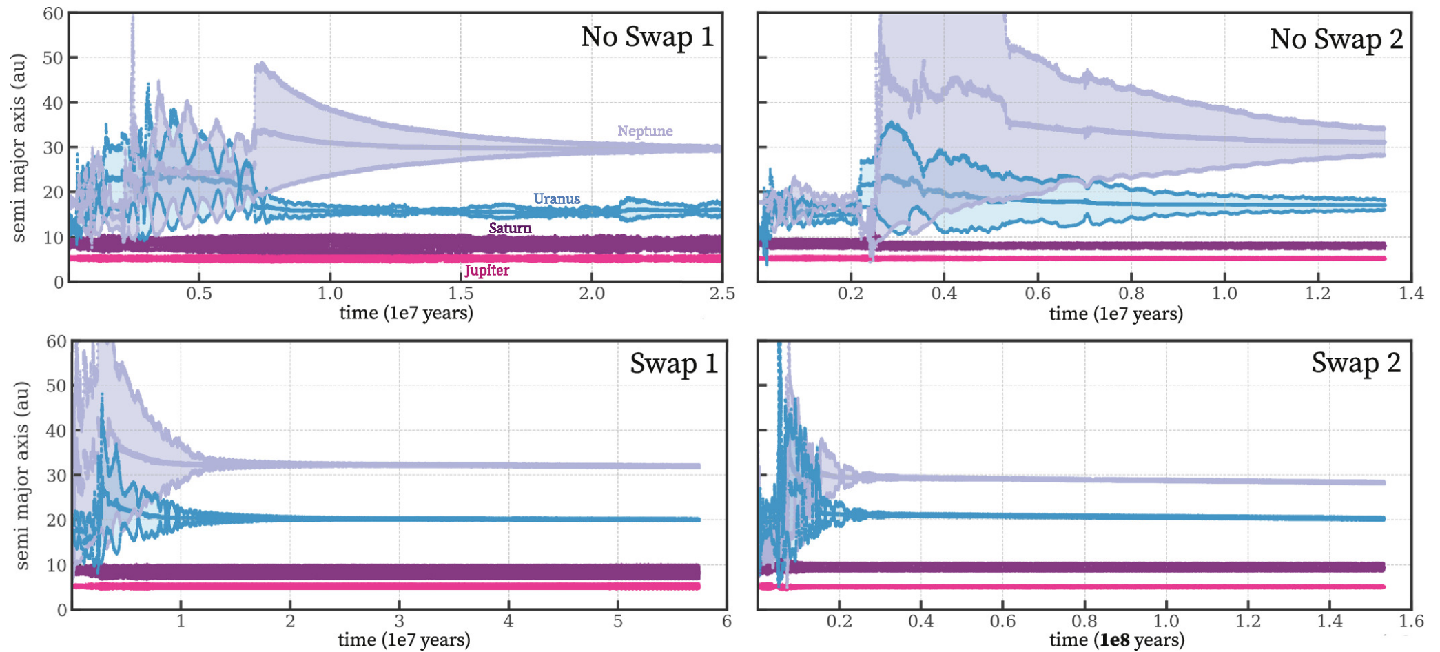
Figure 9. from Eva Zlimen et al 2024 Astron. J. 168 doi:10.3847/1538-3881/ad4c6a https://dx.doi.org/10.3847/1538-3881/ad4c6a © 2024. The Author(s). Published by the American Astronomical Society.
