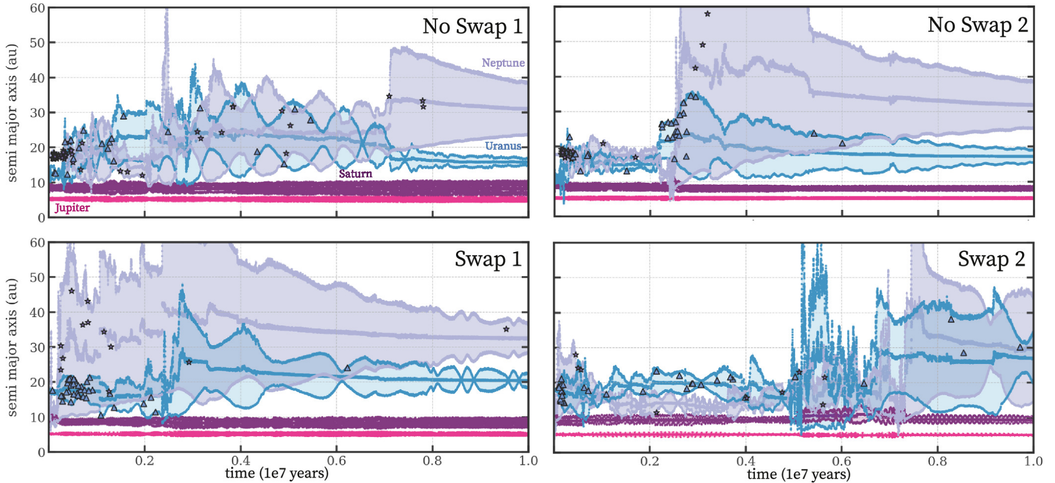
Figure 8. from Eva Zlimen et al 2024 Astron. J. 168 doi:10.3847/1538-3881/ad4c6a https://dx.doi.org/10.3847/1538-3881/ad4c6a © 2024. The Author(s). Published by the American Astronomical Society.
