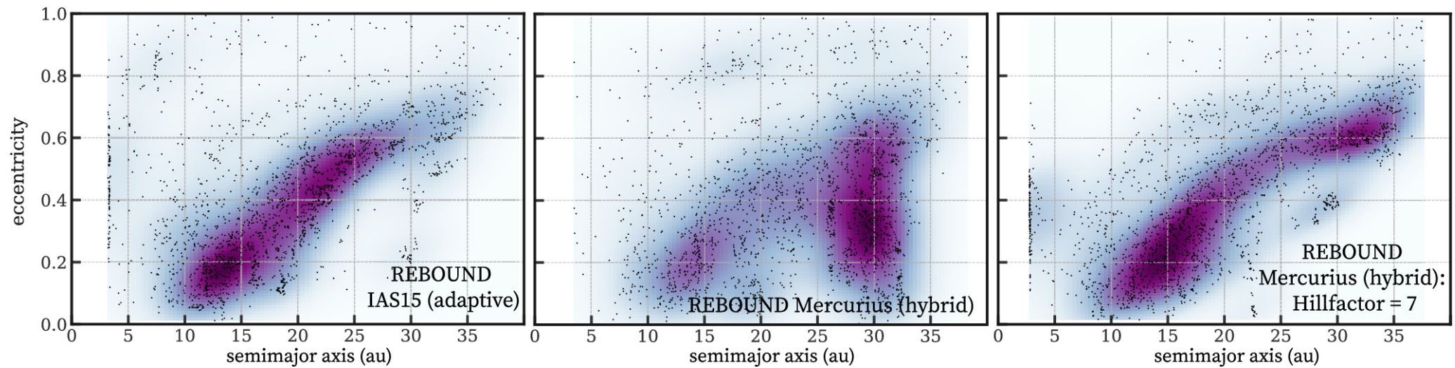
Figure 7. from Eva Zlimen et al 2024 Astron. J. 168 doi:10.3847/1538-3881/ad4c6a https://dx.doi.org/10.3847/1538-3881/ad4c6a © 2024. The Author(s). Published by the American Astronomical Society.
