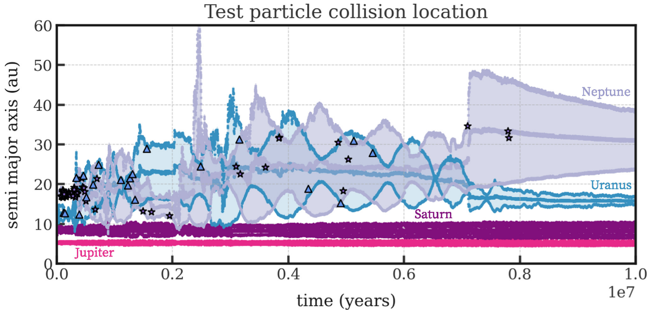
Figure 4. from Eva Zlimen et al 2024 Astron. J. 168 doi:10.3847/1538-3881/ad4c6a https://dx.doi.org/10.3847/1538-3881/ad4c6a © 2024. The Author(s). Published by the American Astronomical Society.
