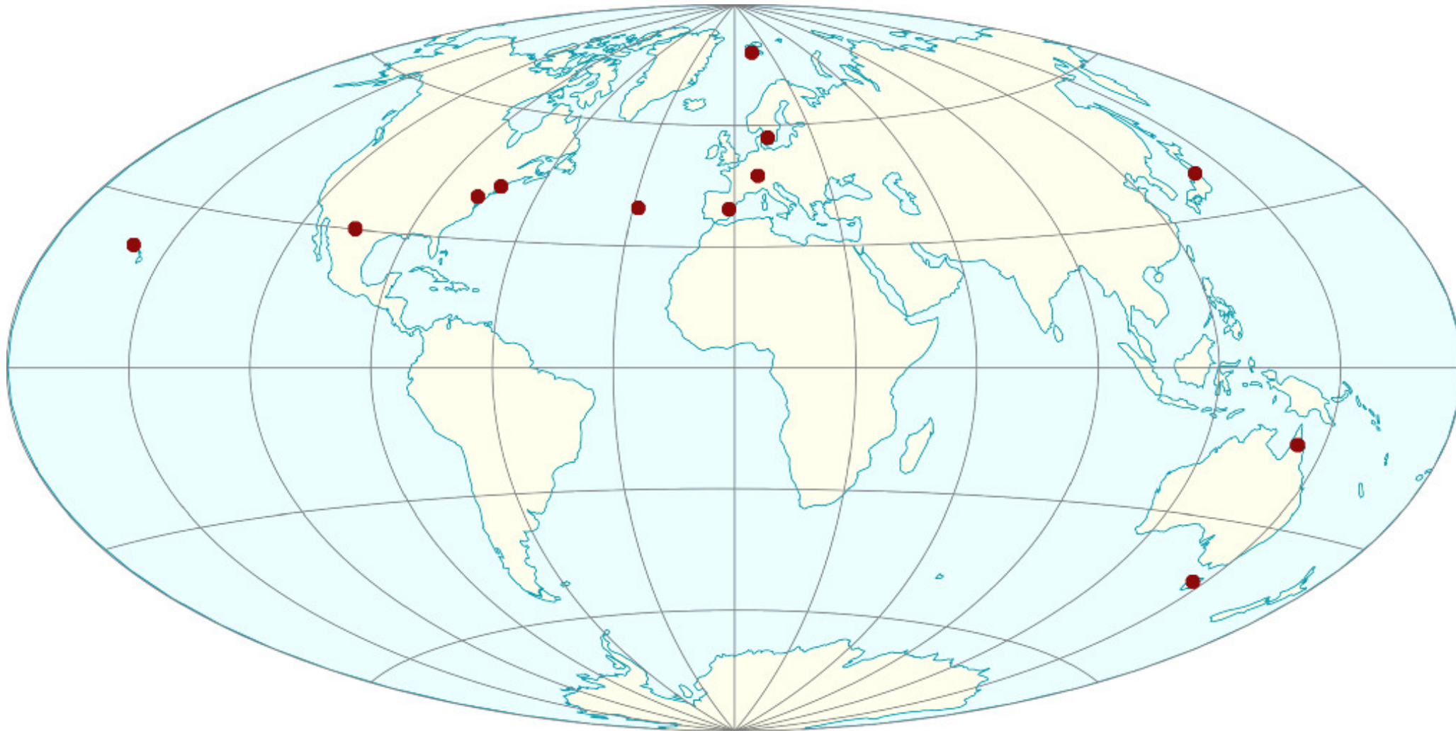
Figure 4. from Leonid Petrov 2024 Astron. J. 168 doi:10.3847/1538-3881/ad4a6b https://dx.doi.org/10.3847/1538-3881/ad4a6b © 2024. The Author(s). Published by the American Astronomical Society.
