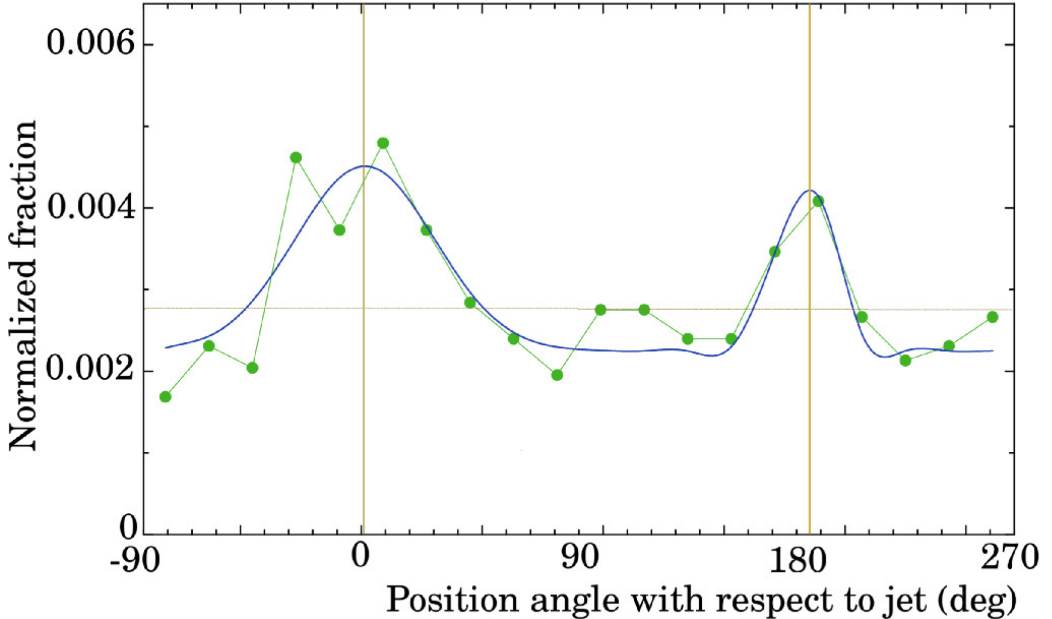
Figure 21. from Leonid Petrov 2024 Astron. J. 168 doi:10.3847/1538-3881/ad4a6b https://dx.doi.org/10.3847/1538-3881/ad4a6b © 2024. The Author(s). Published by the American Astronomical Society.
