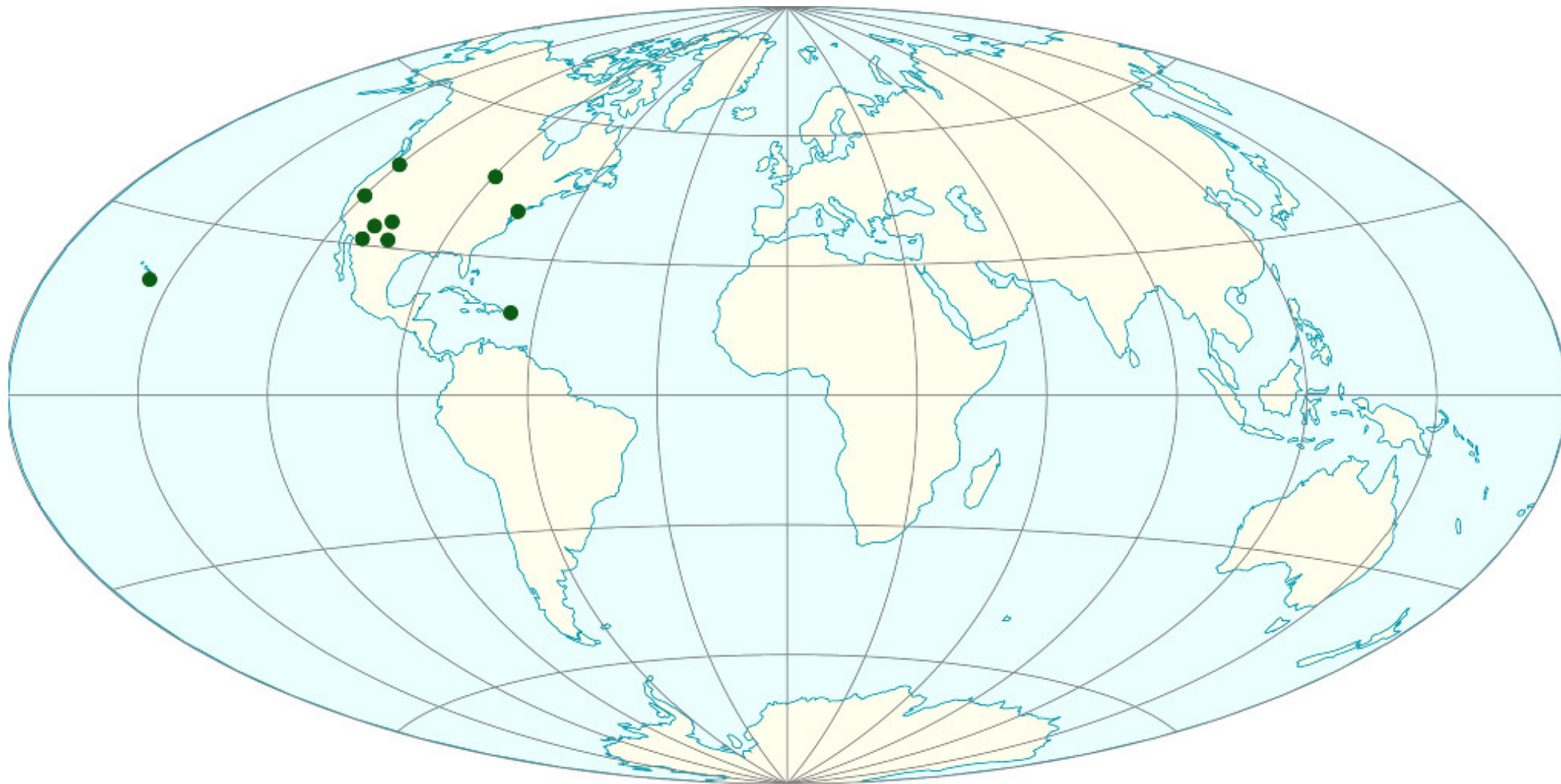
Figure 2. from Leonid Petrov 2024 Astron. J. 168 doi:10.3847/1538-3881/ad4a6b https://dx.doi.org/10.3847/1538-3881/ad4a6b © 2024. The Author(s). Published by the American Astronomical Society.
