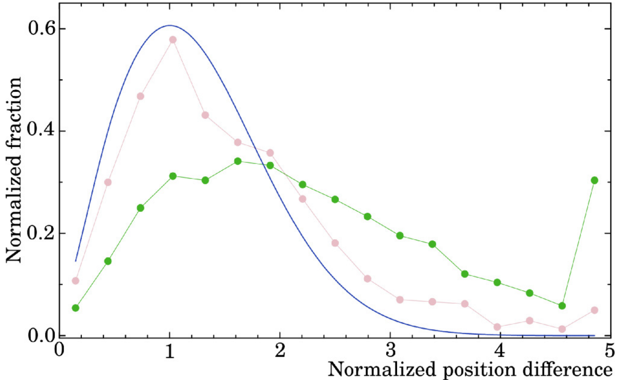
Figure 17. from Leonid Petrov 2024 Astron. J. 168 doi:10.3847/1538-3881/ad4a6b https://dx.doi.org/10.3847/1538-3881/ad4a6b © 2024. The Author(s). Published by the American Astronomical Society.
