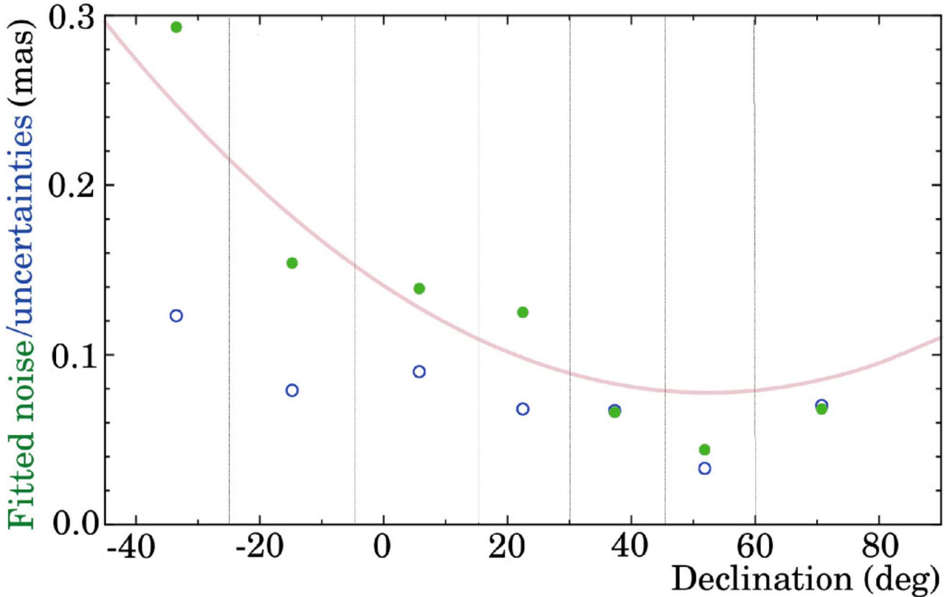
Figure 16. from Leonid Petrov 2024 Astron. J. 168 doi:10.3847/1538-3881/ad4a6b https://dx.doi.org/10.3847/1538-3881/ad4a6b © 2024. The Author(s). Published by the American Astronomical Society.
