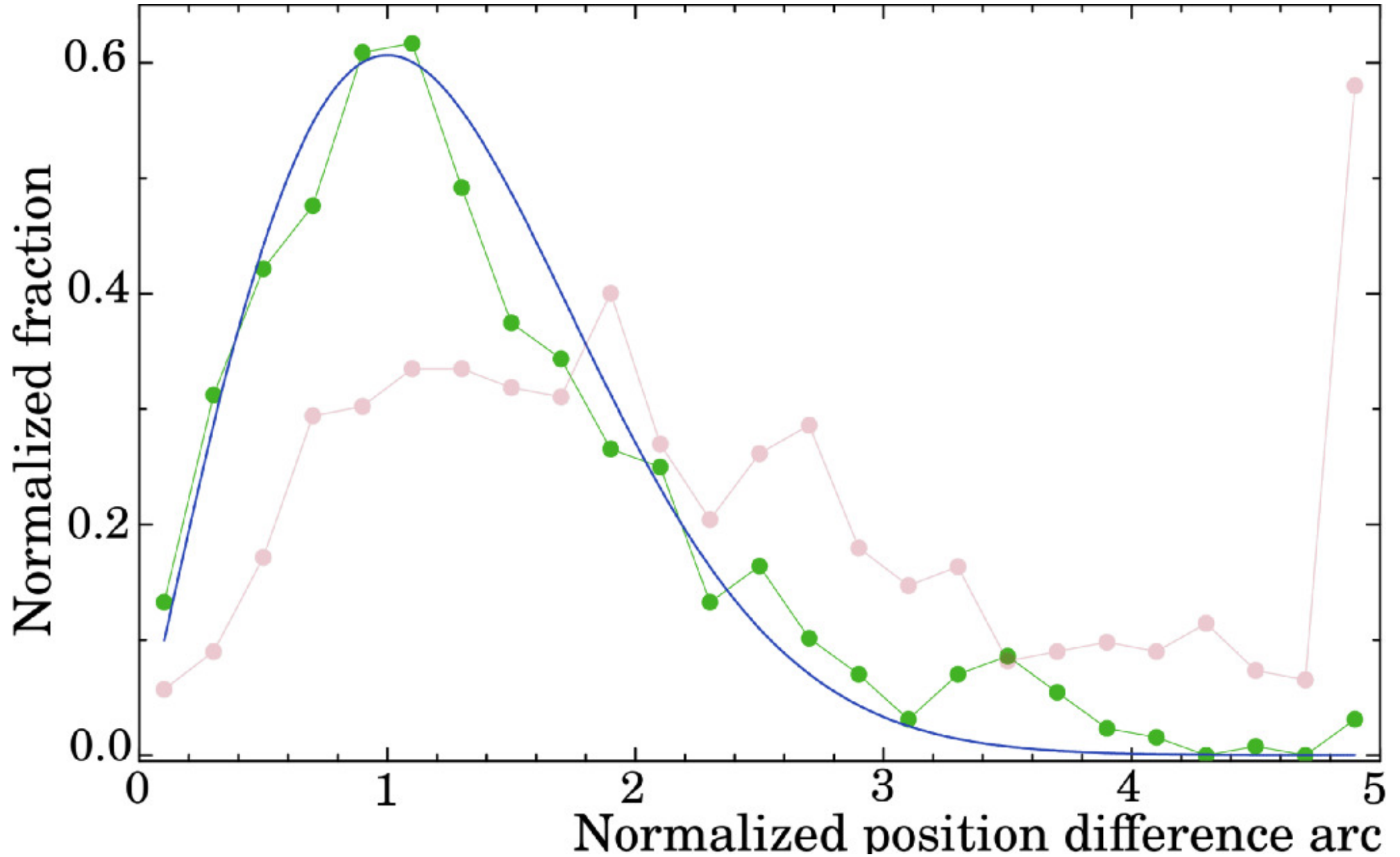
Figure 13. from Leonid Petrov 2024 Astron. J. 168 doi:10.3847/1538-3881/ad4a6b https://dx.doi.org/10.3847/1538-3881/ad4a6b © 2024. The Author(s). Published by the American Astronomical Society.
