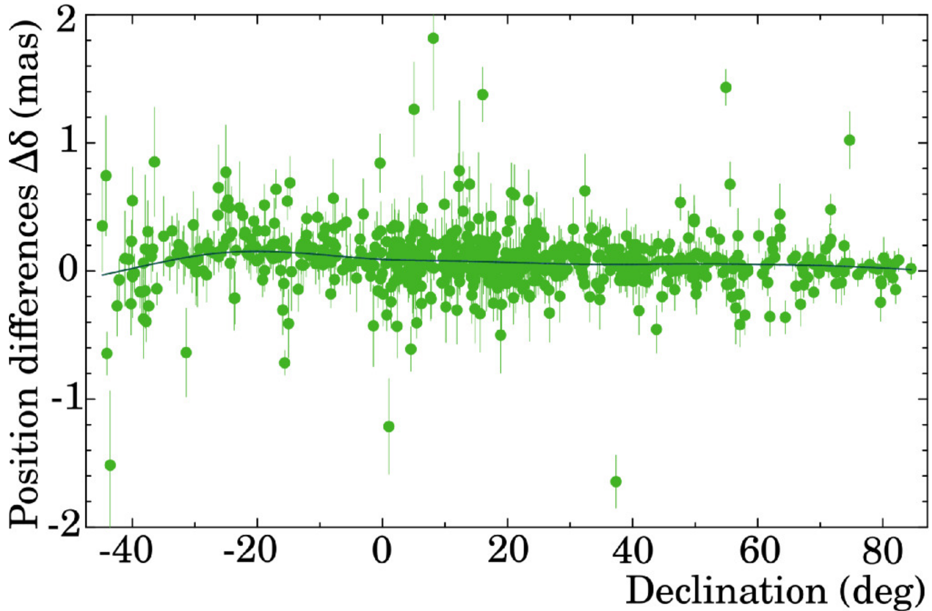
Figure 12. from Leonid Petrov 2024 Astron. J. 168 doi:10.3847/1538-3881/ad4a6b https://dx.doi.org/10.3847/1538-3881/ad4a6b © 2024. The Author(s). Published by the American Astronomical Society.
