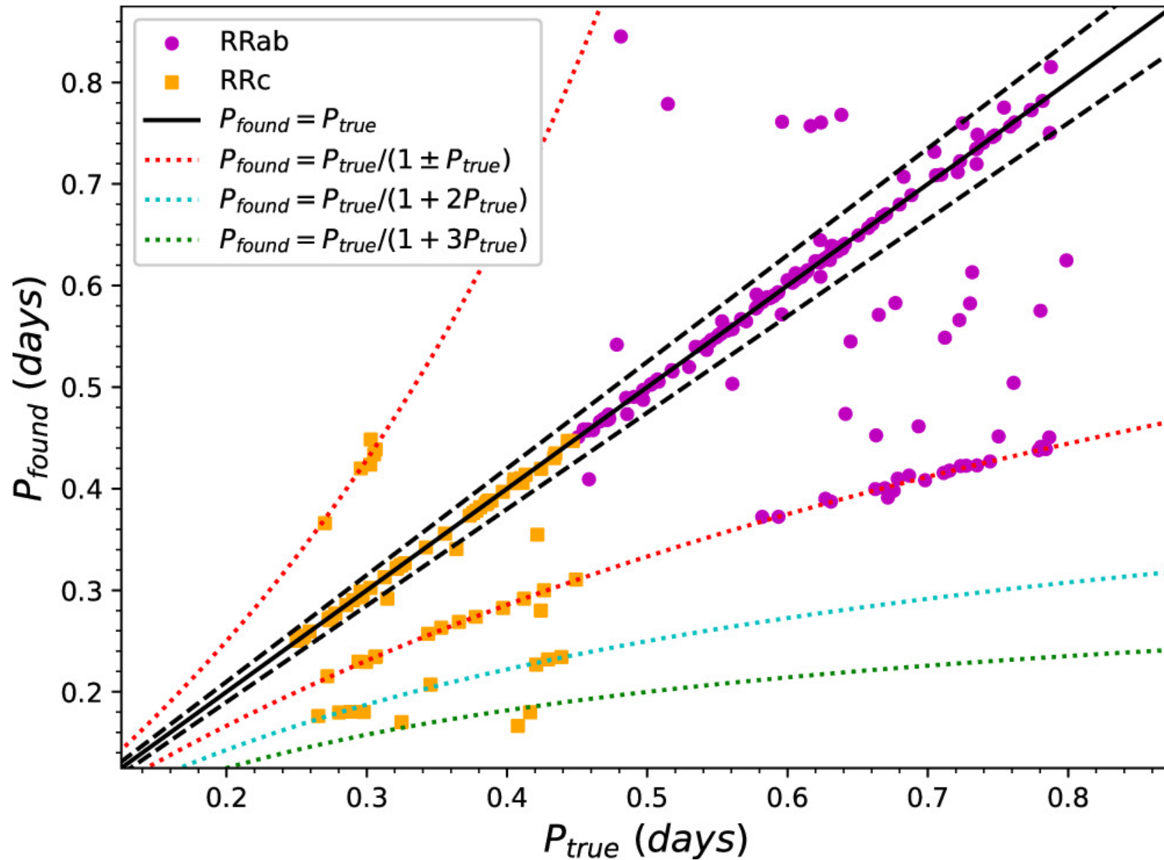
Figure 2. from Chow-Choong Ngeow and Anupam Bhardwaj 2024 Astron. J. 168 doi:10.3847/1538-3881/ad49a9 https://dx.doi.org/10.3847/1538-3881/ad49a9 © 2024. The Author(s). Published by the American Astronomical Society.
