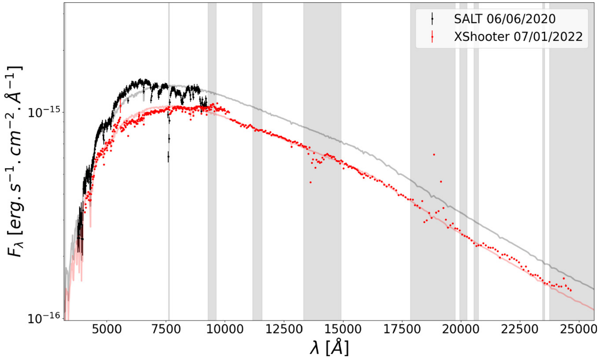
Figure 3. from E. Bachelet et al 2024 Astron. J. 168 doi:10.3847/1538-3881/ad46fc https://dx.doi.org/10.3847/1538-3881/ad46fc © 2024. The Author(s). Published by the American Astronomical Society.
