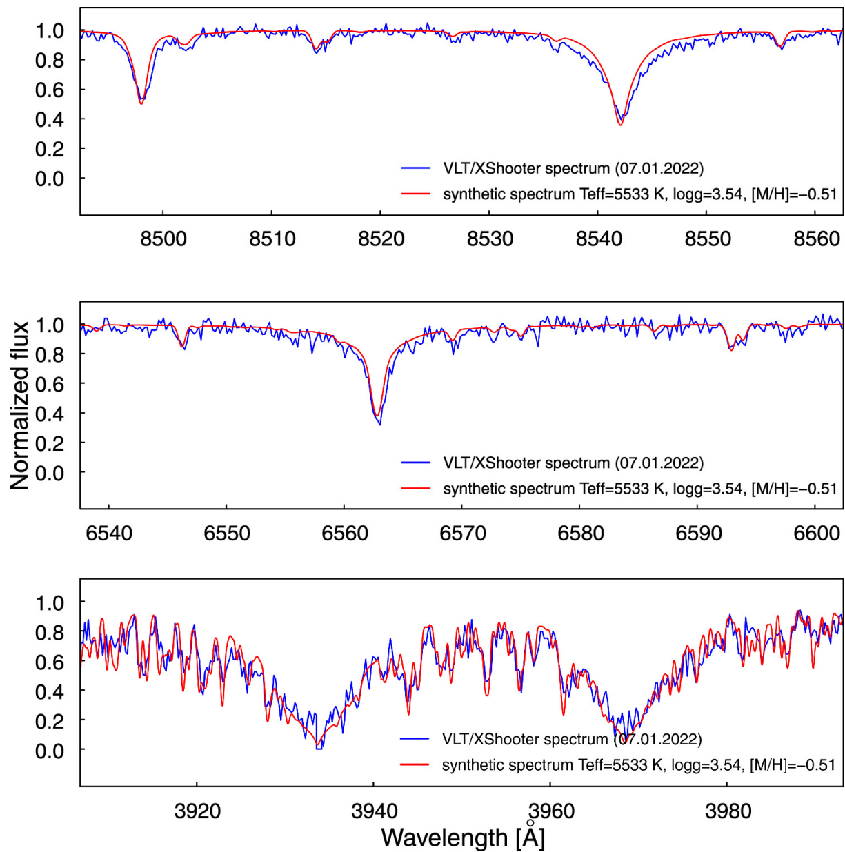
Figure 2. from E. Bachelet et al 2024 Astron. J. 168 doi:10.3847/1538-3881/ad46fc https://dx.doi.org/10.3847/1538-3881/ad46fc © 2024. The Author(s). Published by the American Astronomical Society.
