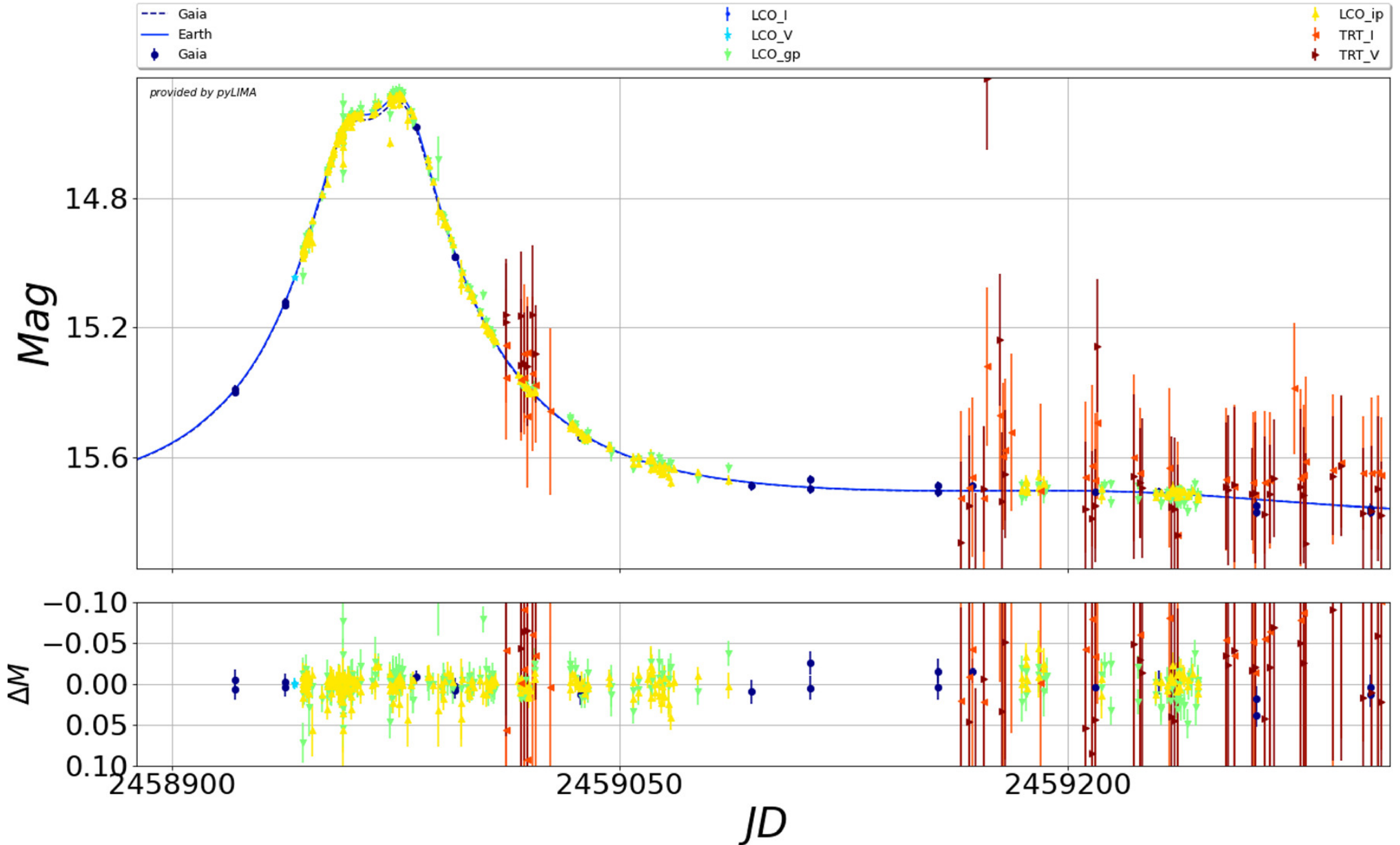
Figure 1. from E. Bachelet et al 2024 Astron. J. 168 doi:10.3847/1538-3881/ad46fc https://dx.doi.org/10.3847/1538-3881/ad46fc © 2024. The Author(s). Published by the American Astronomical Society.
