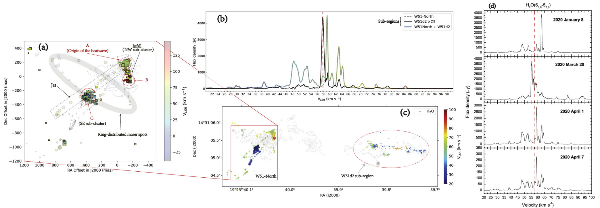
Figure 9. from Yan-Kun Zhang et al 2024 Astron. J. 168 doi:10.3847/1538-3881/ad428d https://dx.doi.org/10.3847/1538-3881/ad428d © 2024. The Author(s). Published by the American Astronomical Society.
