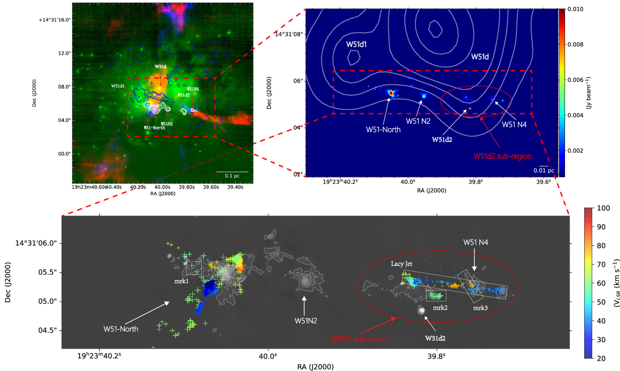
Figure 8. from Yan-Kun Zhang et al 2024 Astron. J. 168 doi:10.3847/1538-3881/ad428d https://dx.doi.org/10.3847/1538-3881/ad428d © 2024. The Author(s). Published by the American Astronomical Society.
