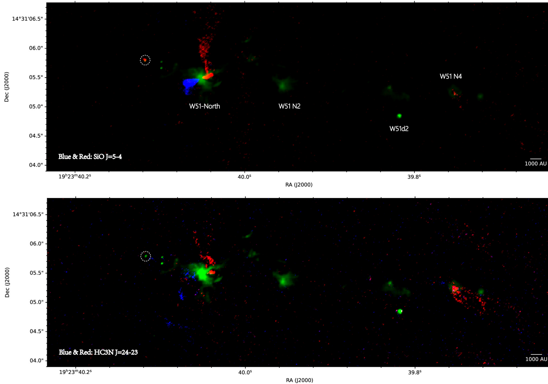
Figure 5. from Yan-Kun Zhang et al 2024 Astron. J. 168 doi:10.3847/1538-3881/ad428d https://dx.doi.org/10.3847/1538-3881/ad428d © 2024. The Author(s). Published by the American Astronomical Society.
