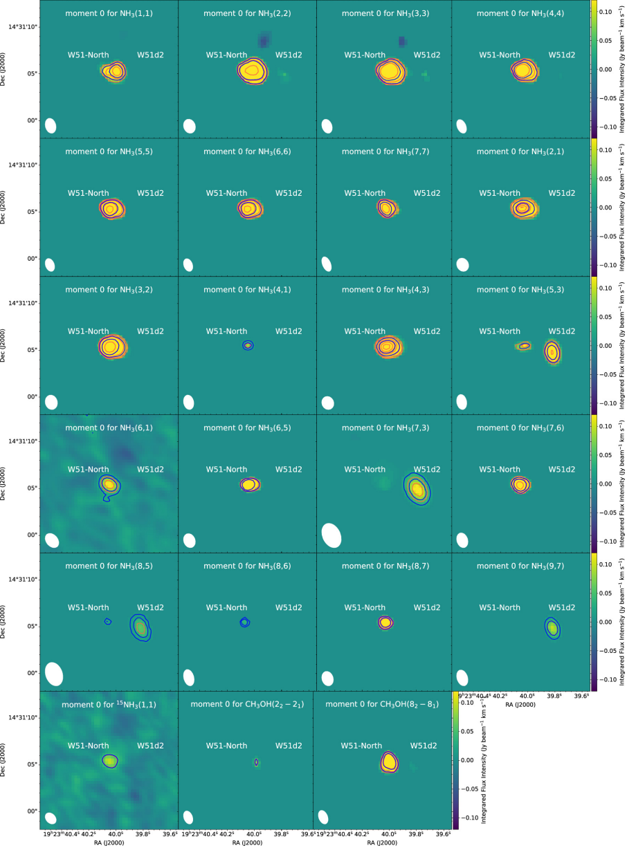
Figure 4. from Yan-Kun Zhang et al 2024 Astron. J. 168 doi:10.3847/1538-3881/ad428d https://dx.doi.org/10.3847/1538-3881/ad428d © 2024. The Author(s). Published by the American Astronomical Society.
