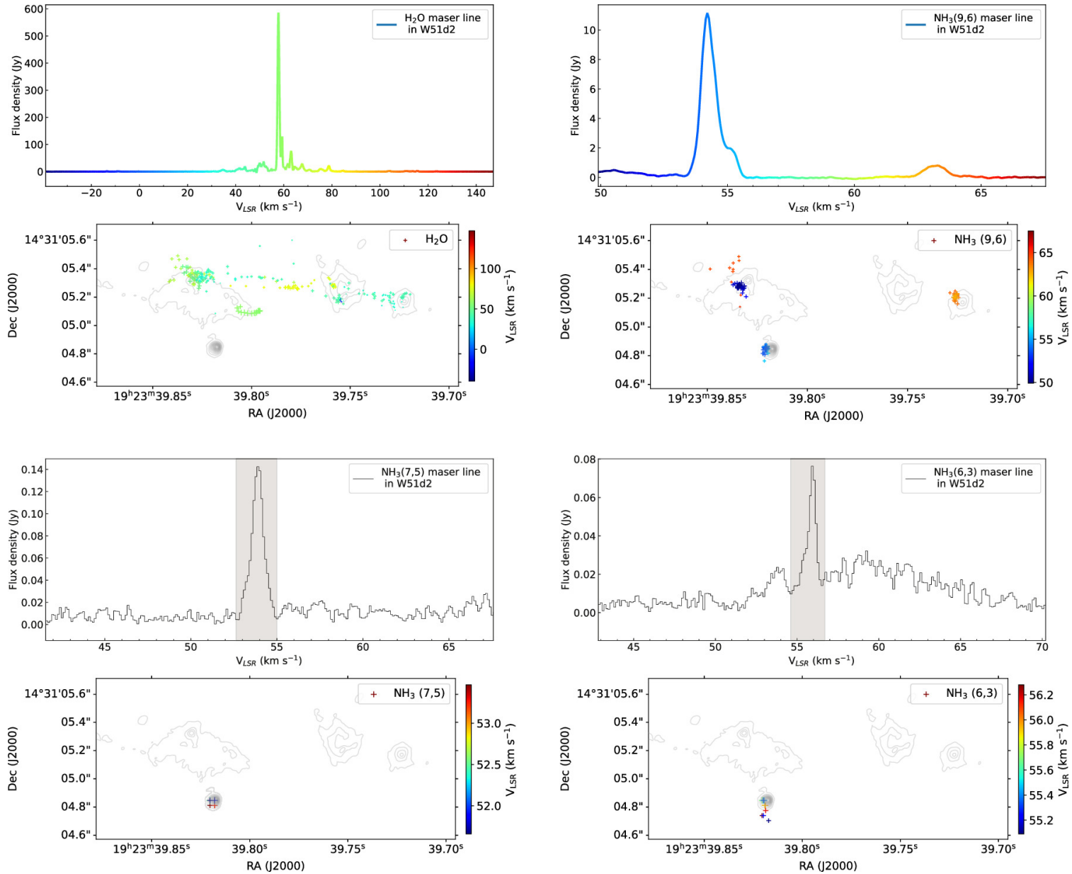
Figure 3. from Yan-Kun Zhang et al 2024 Astron. J. 168 doi:10.3847/1538-3881/ad428d https://dx.doi.org/10.3847/1538-3881/ad428d © 2024. The Author(s). Published by the American Astronomical Society.
