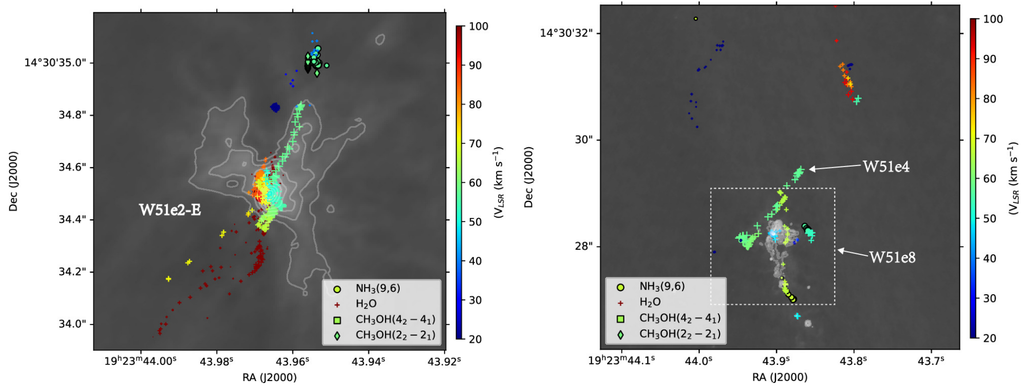
Figure 13. from Yan-Kun Zhang et al 2024 Astron. J. 168 doi:10.3847/1538-3881/ad428d https://dx.doi.org/10.3847/1538-3881/ad428d © 2024. The Author(s). Published by the American Astronomical Society.
