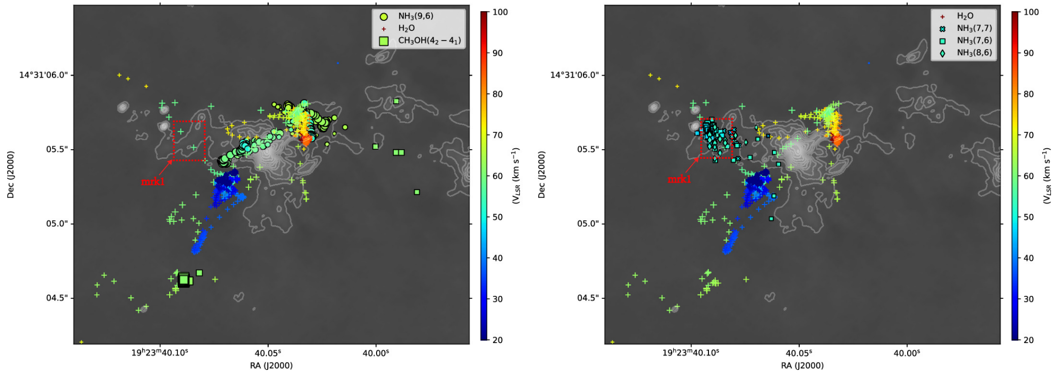
Figure 11. from Yan-Kun Zhang et al 2024 Astron. J. 168 doi:10.3847/1538-3881/ad428d https://dx.doi.org/10.3847/1538-3881/ad428d © 2024. The Author(s). Published by the American Astronomical Society.
