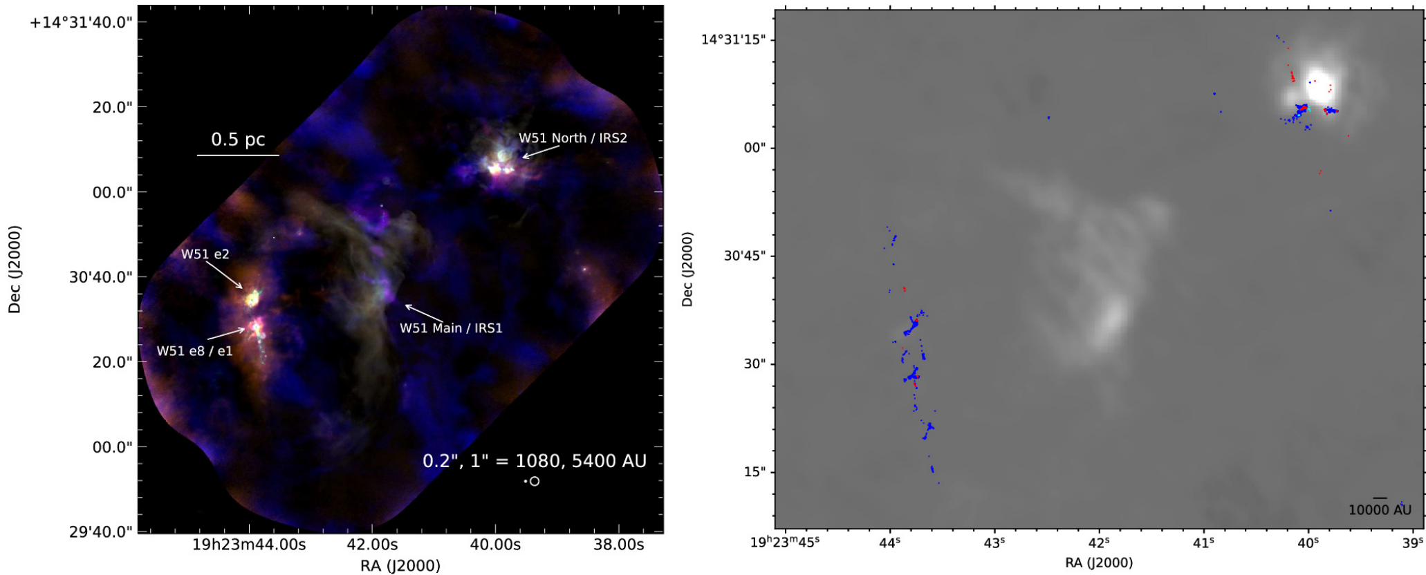
Figure 1. from Yan-Kun Zhang et al 2024 Astron. J. 168 doi:10.3847/1538-3881/ad428d https://dx.doi.org/10.3847/1538-3881/ad428d © 2024. The Author(s). Published by the American Astronomical Society.
