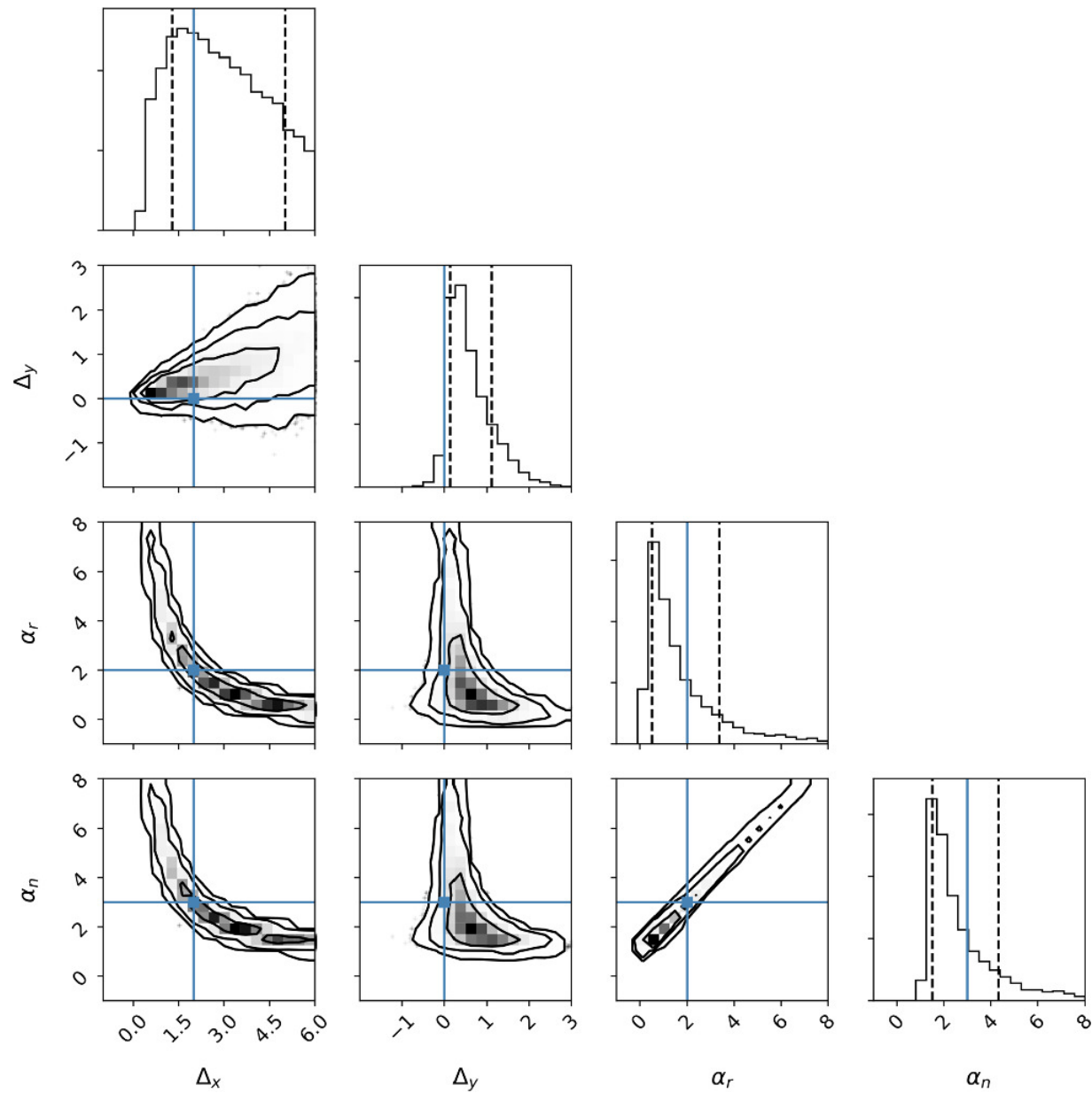
Figure 8. from Ofer Springer et al 2024 Astron. J. 167 doi:10.3847/1538-3881/ad408d https://dx.doi.org/10.3847/1538-3881/ad408d © 2024. The Author(s). Published by the American Astronomical Society.
